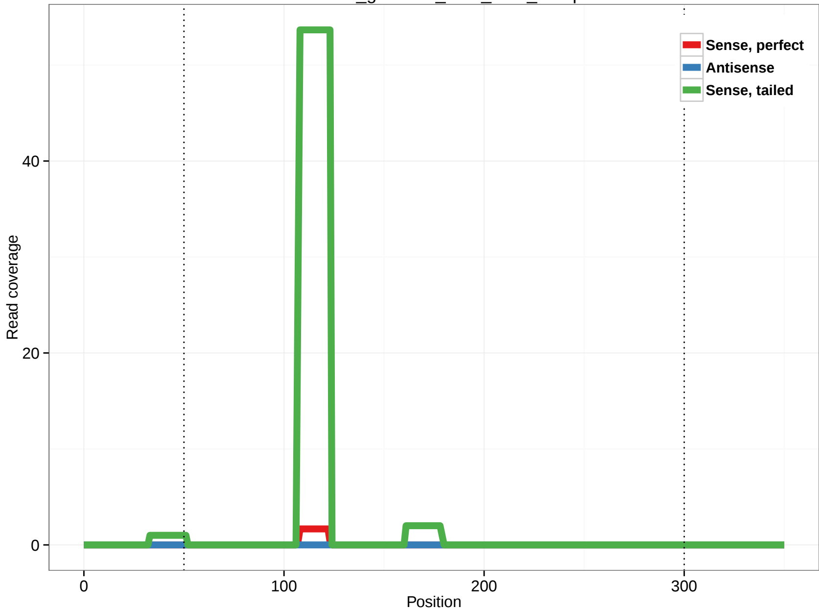
rheMac3_genscan_chr3_05.6_15.5p
