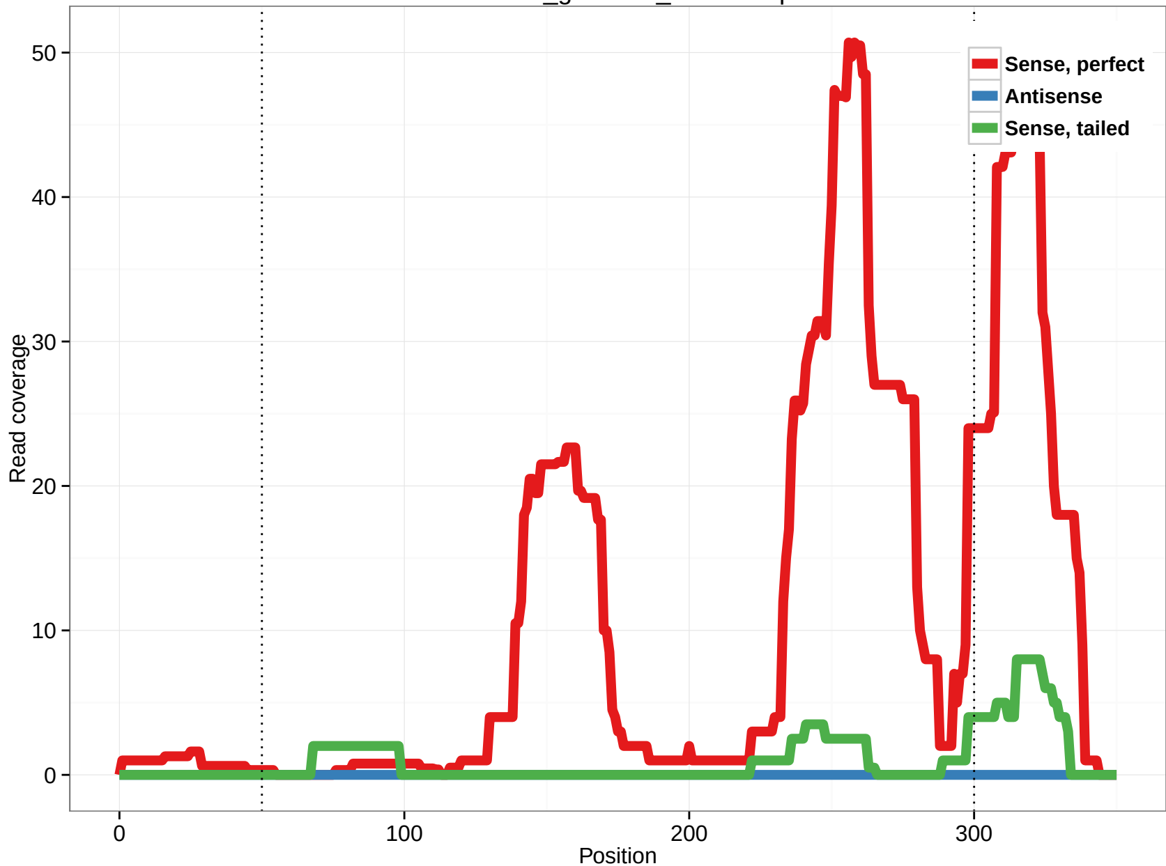
rheMac3_genscan_chr3.12.5p
