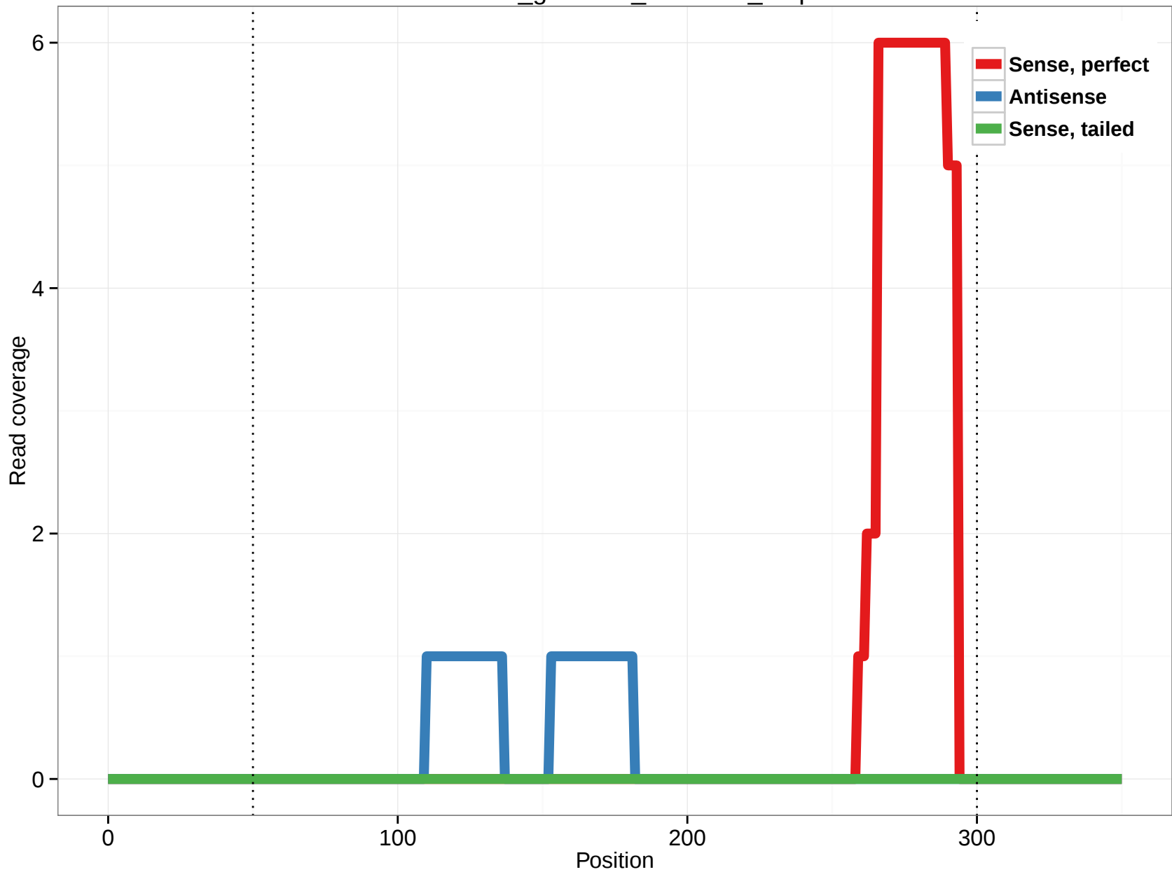
rheMac3_genscan_chr2.979_8.5p
