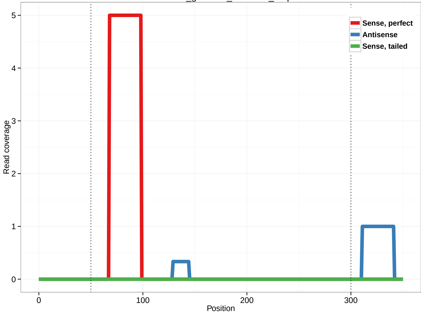
rheMac3_genscan_chr2.979_7.3p
