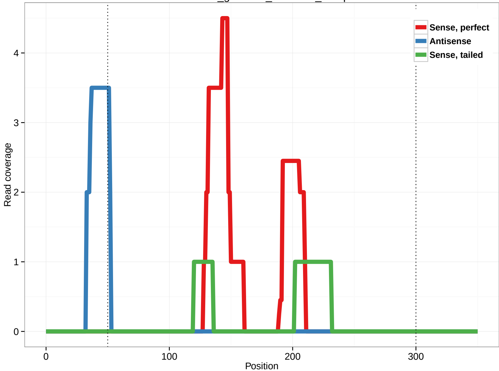
rheMac3_genscan_chr2.891_10.5p
