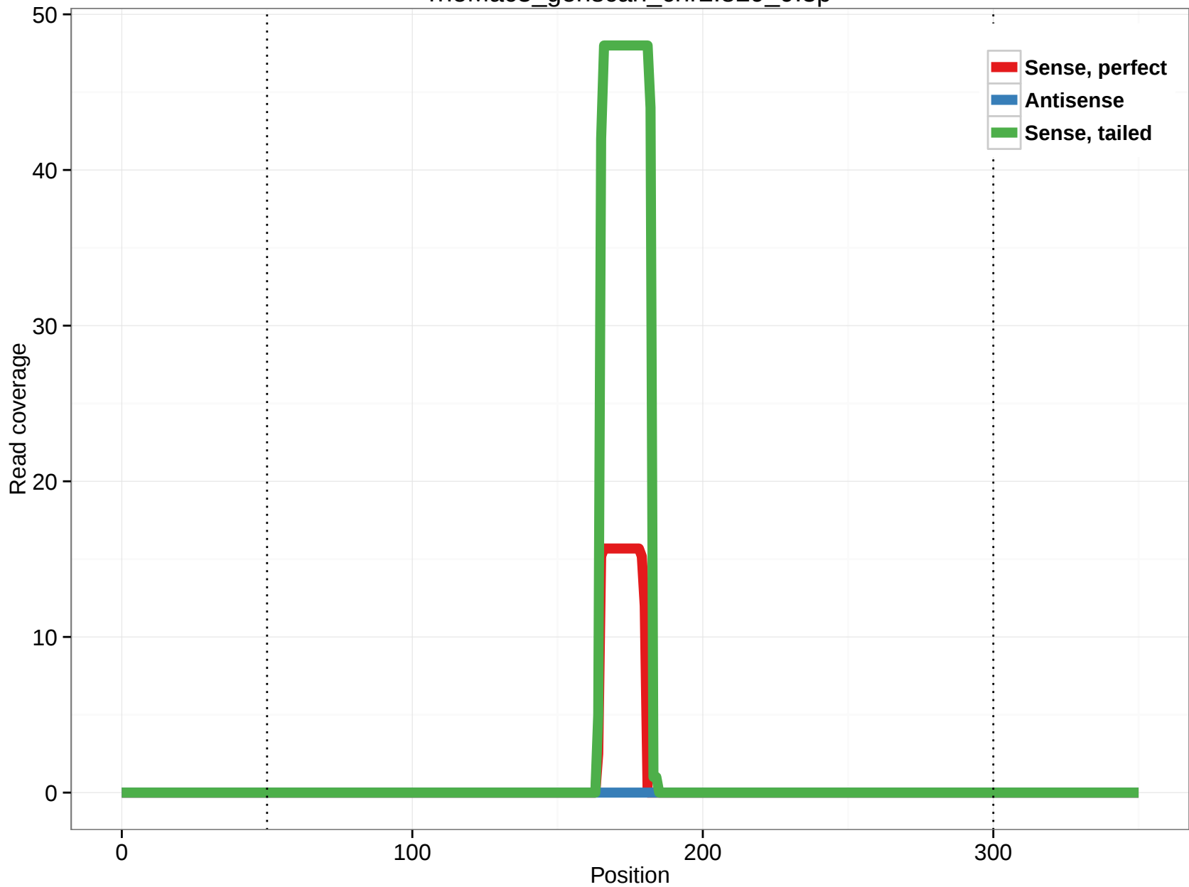
rheMac3_genscan_chr2.829_9.3p
