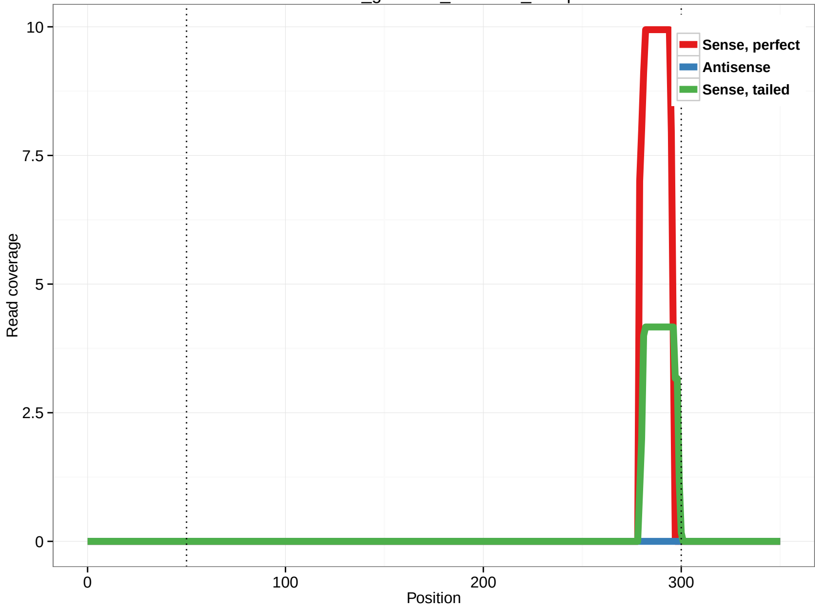
rheMac3_genscan_chr2.749_10.5p
