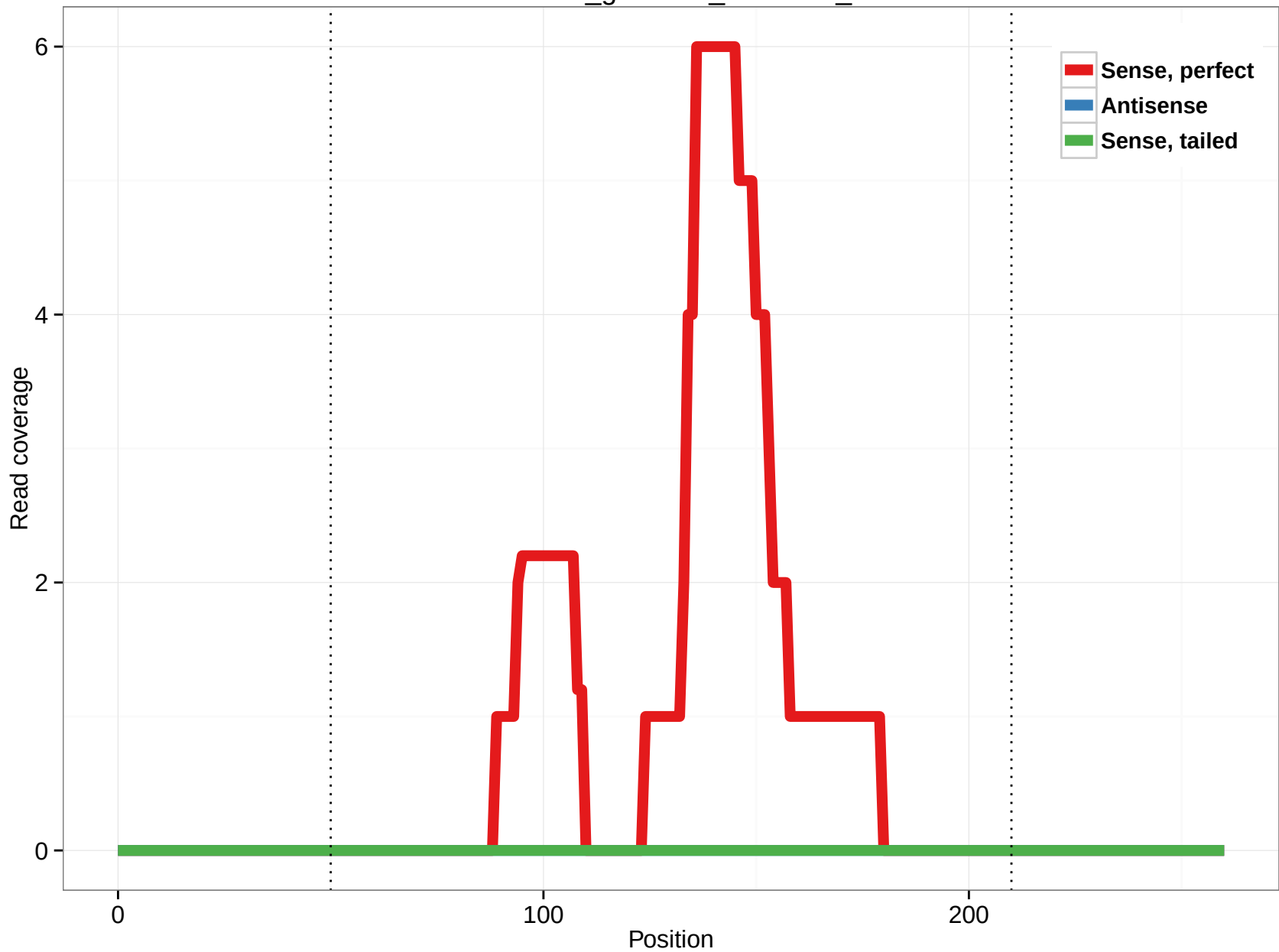
rheMac3_genscan_chr2.726_1
