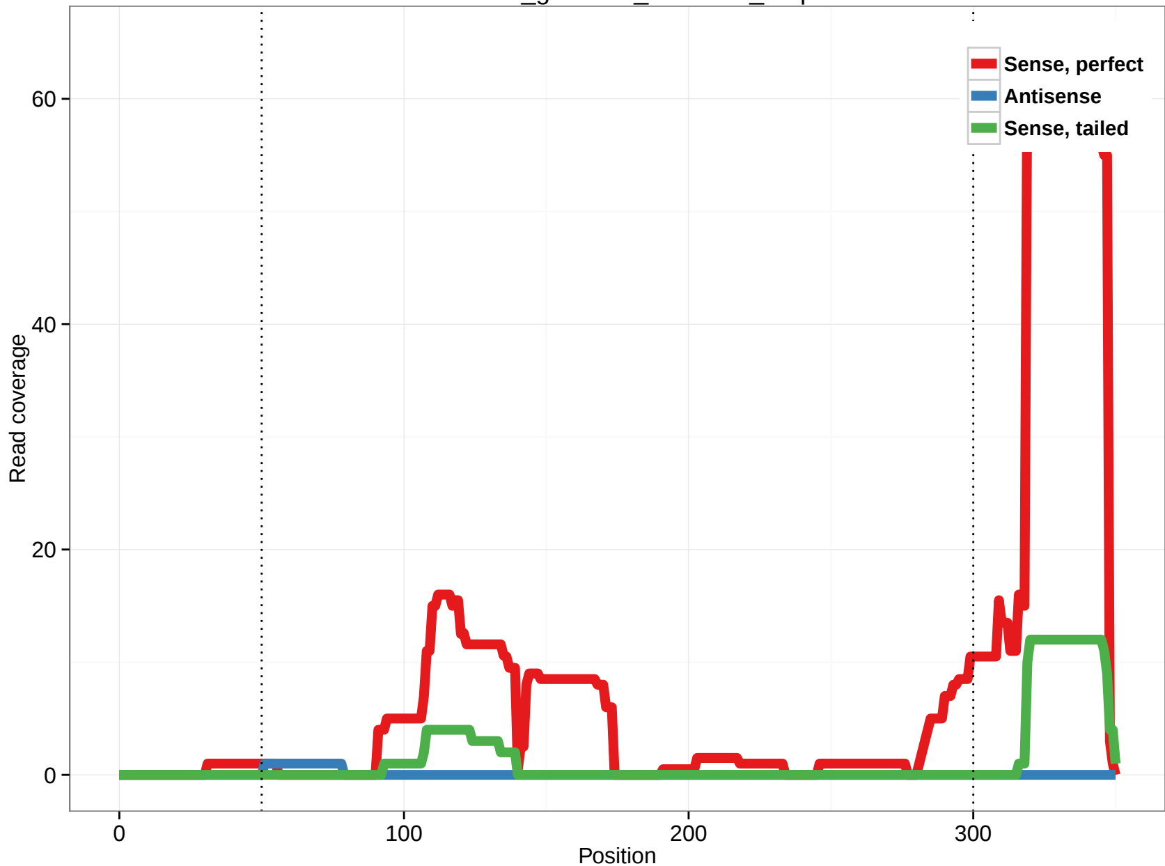
rheMac3_genscan_chr2.697_0.5p
