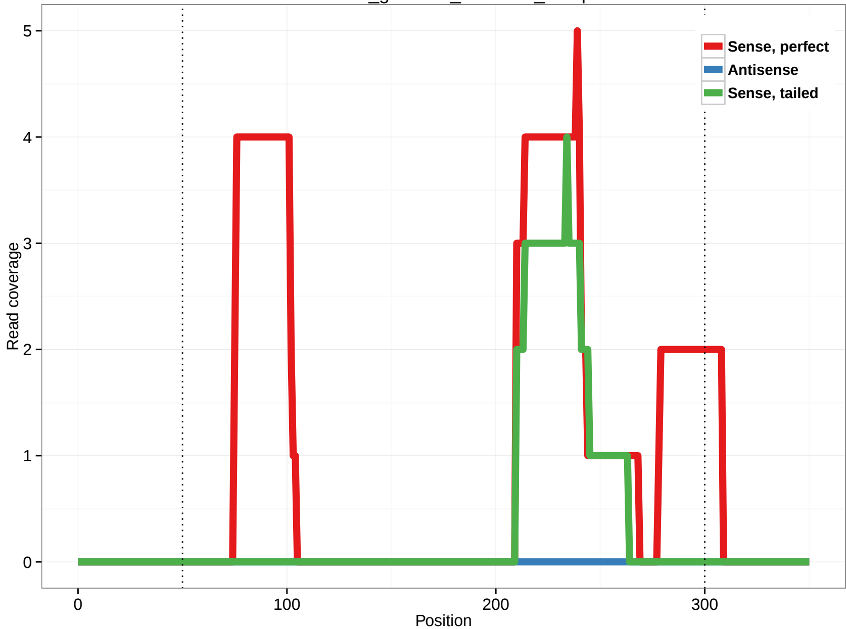
rheMac3_genscan_chr2.622_52.3p
