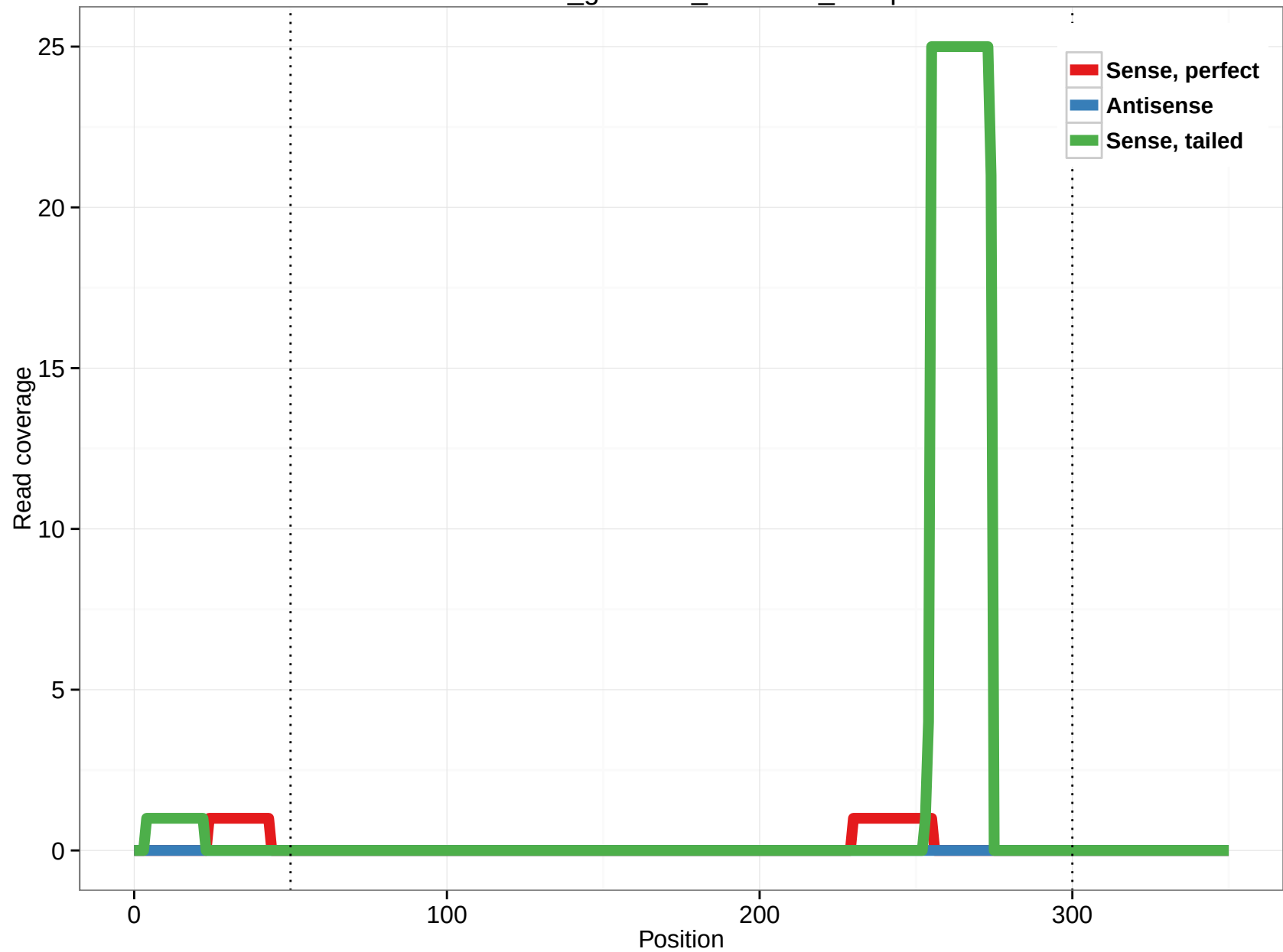
rheMac3_genscan_chr2.578_17.5p
