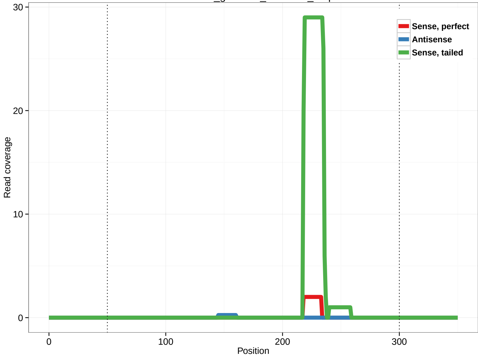
rheMac3_genscan_chr2.551_8.3p
