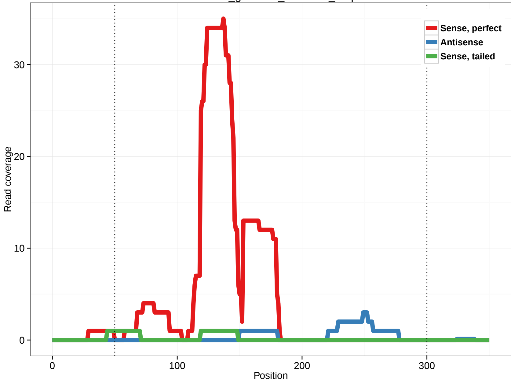
rheMac3_genscan_chr2.521_5.3p
