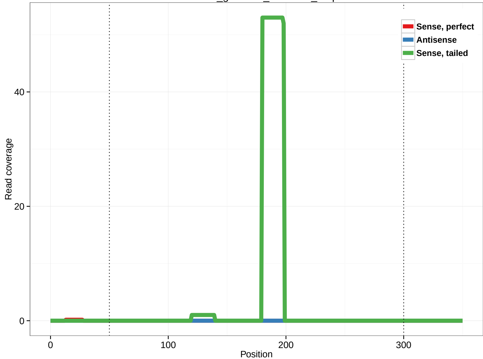
rheMac3_genscan_chr2.505_0.5p
