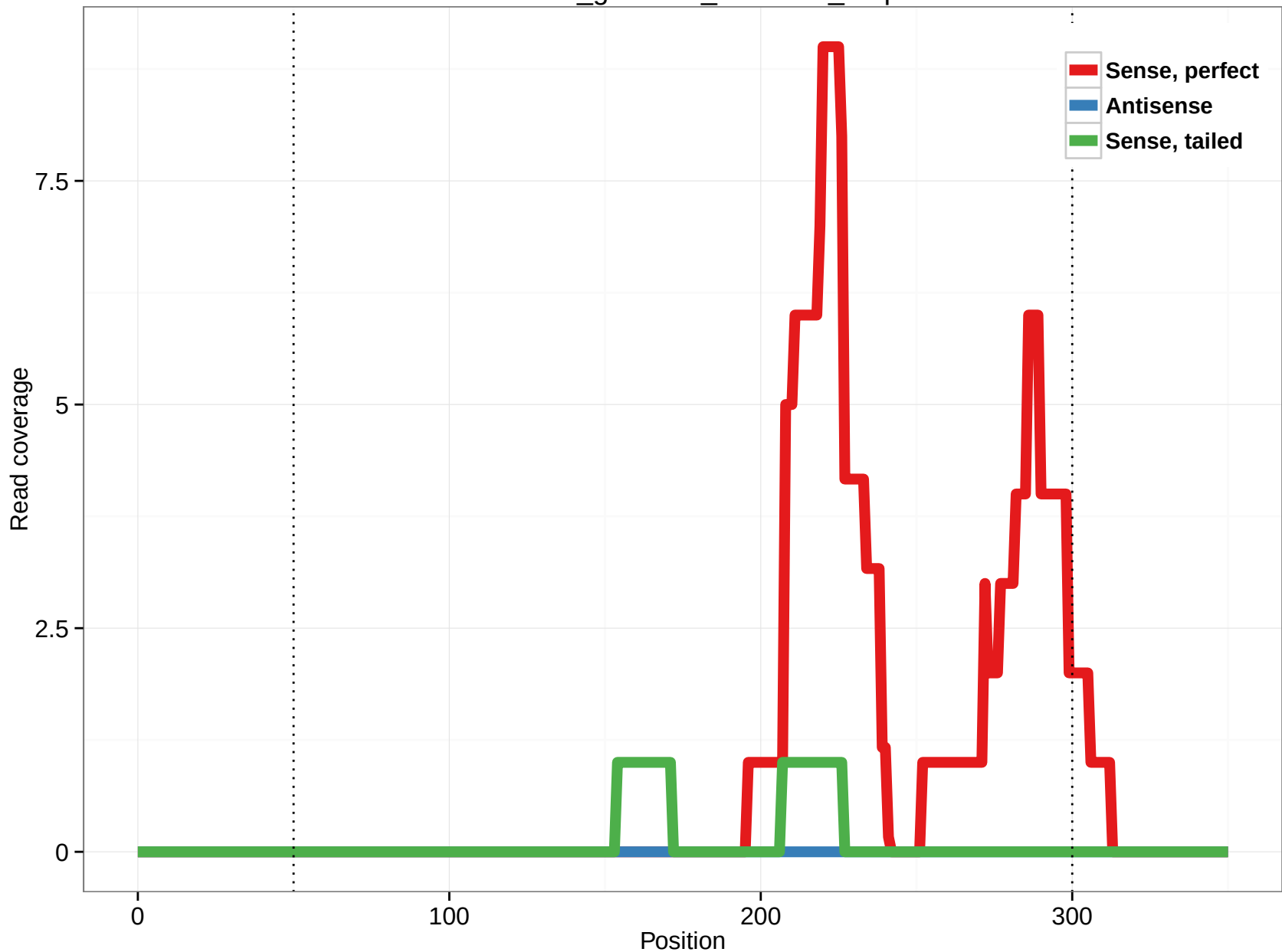
rheMac3_genscan_chr2.440_0.5p
