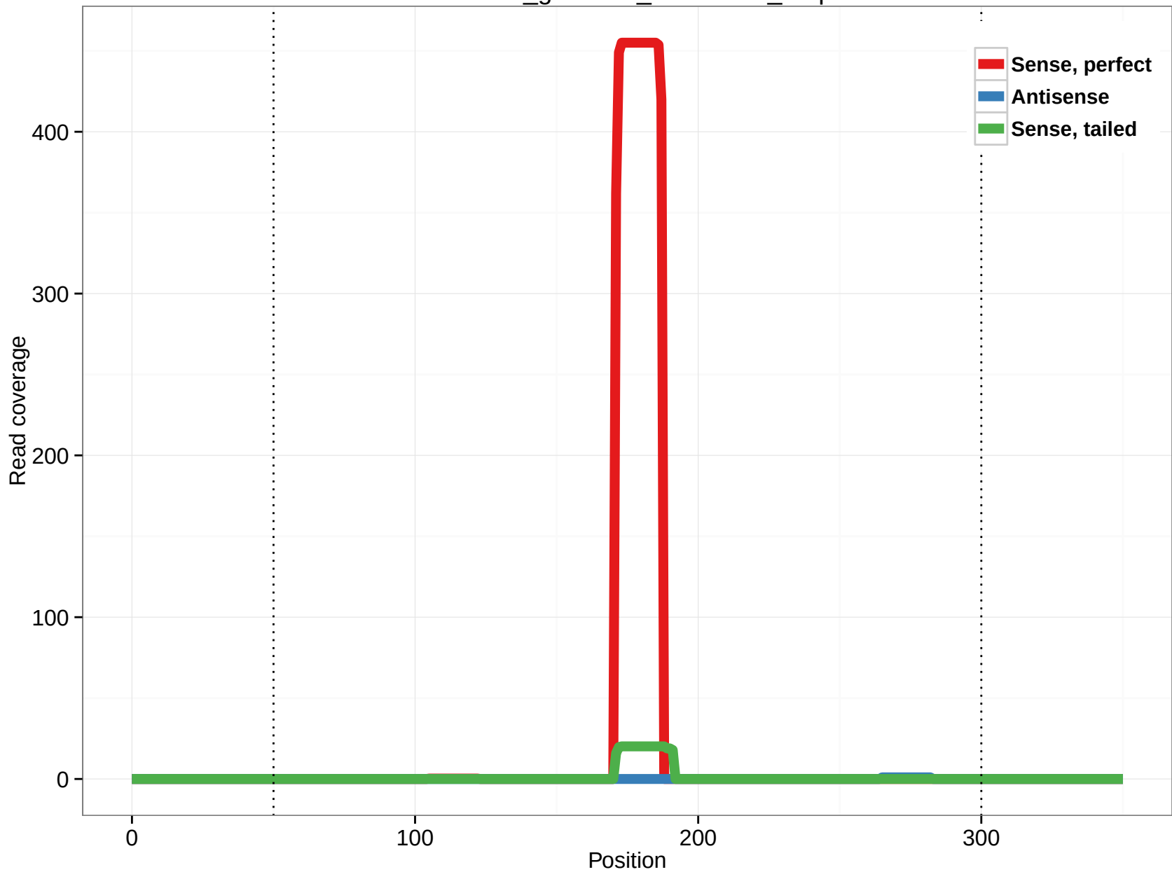
rheMac3_genscan_chr2.3291_2.5p
