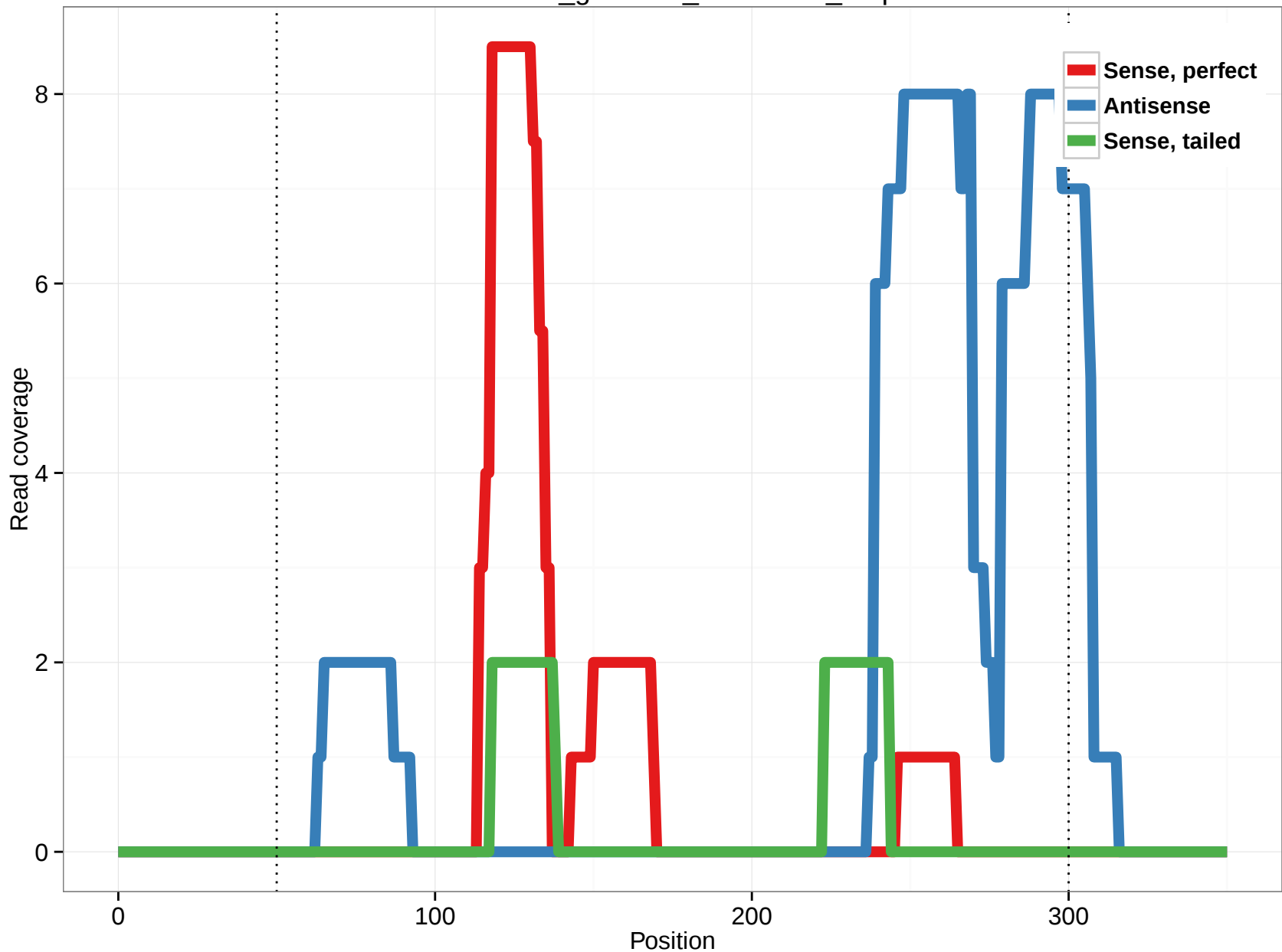
rheMac3_genscan_chr2.3288_5.5p
