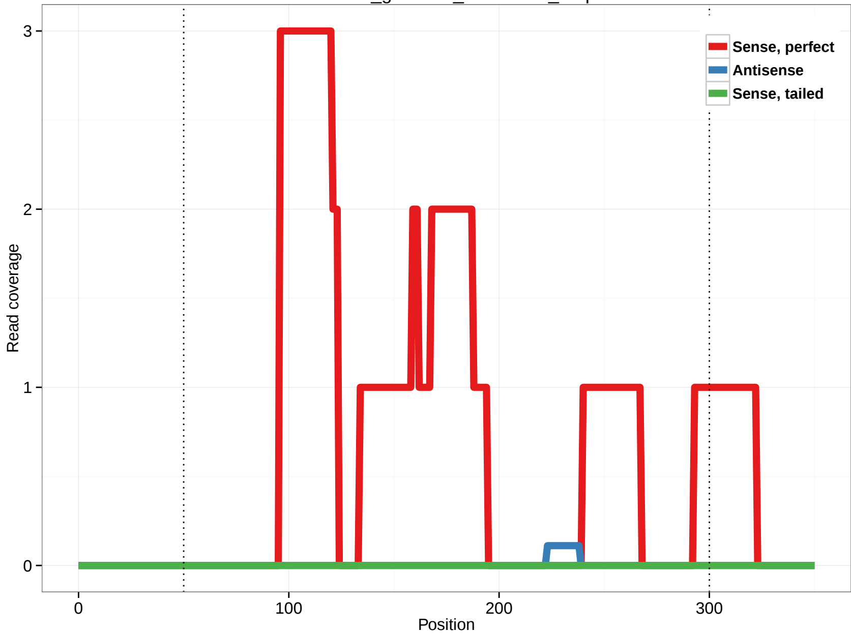
rheMac3_genscan_chr2.3245_1.5p
