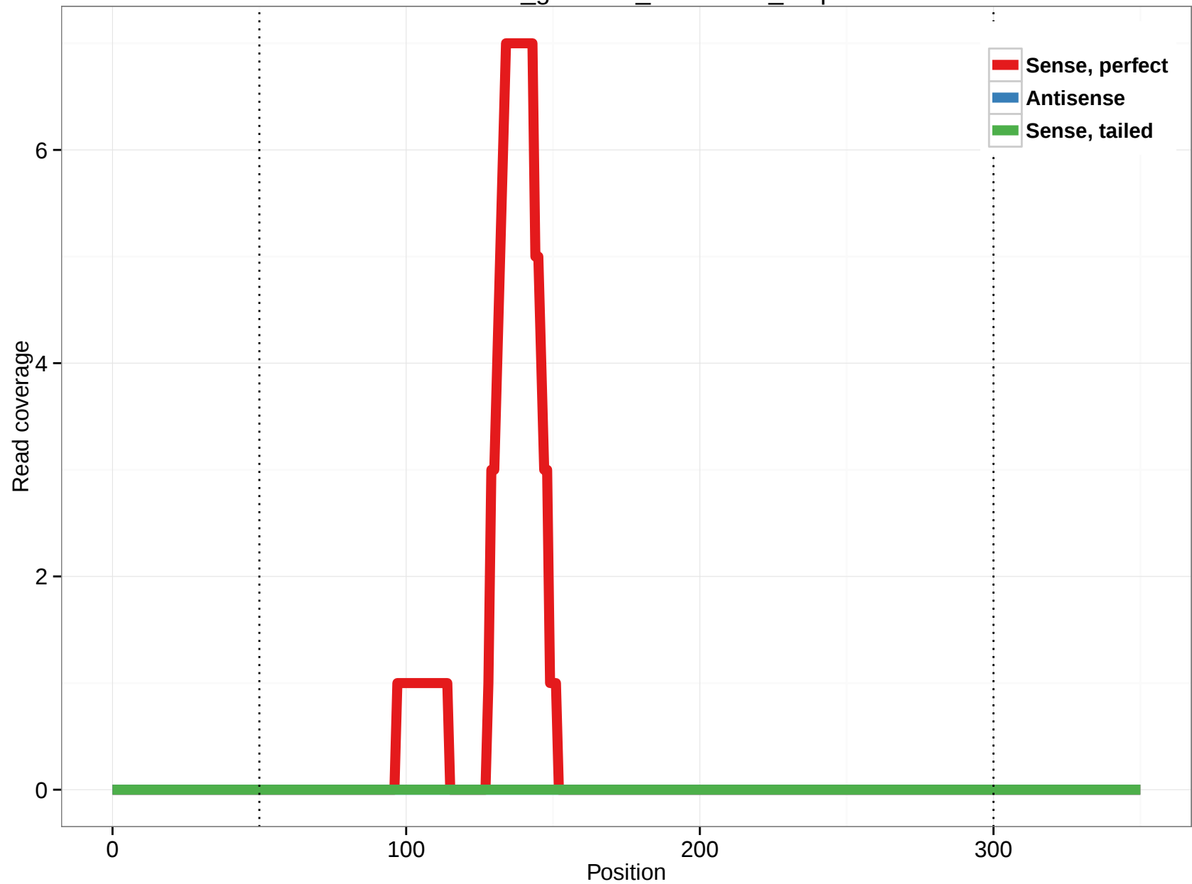
rheMac3_genscan_chr2.3184_2.3p
