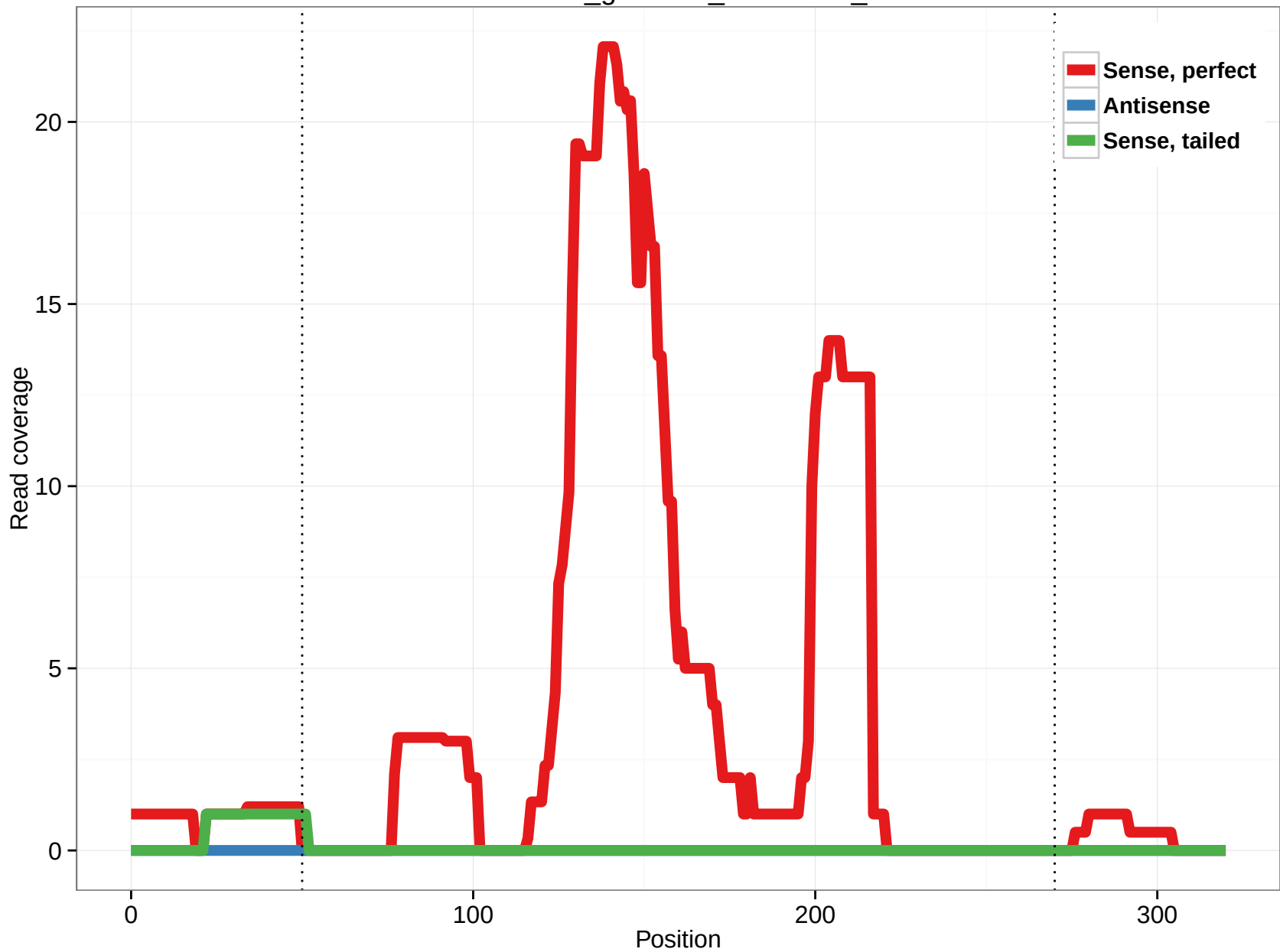
rheMac3_genscan_chr2.3076_8
