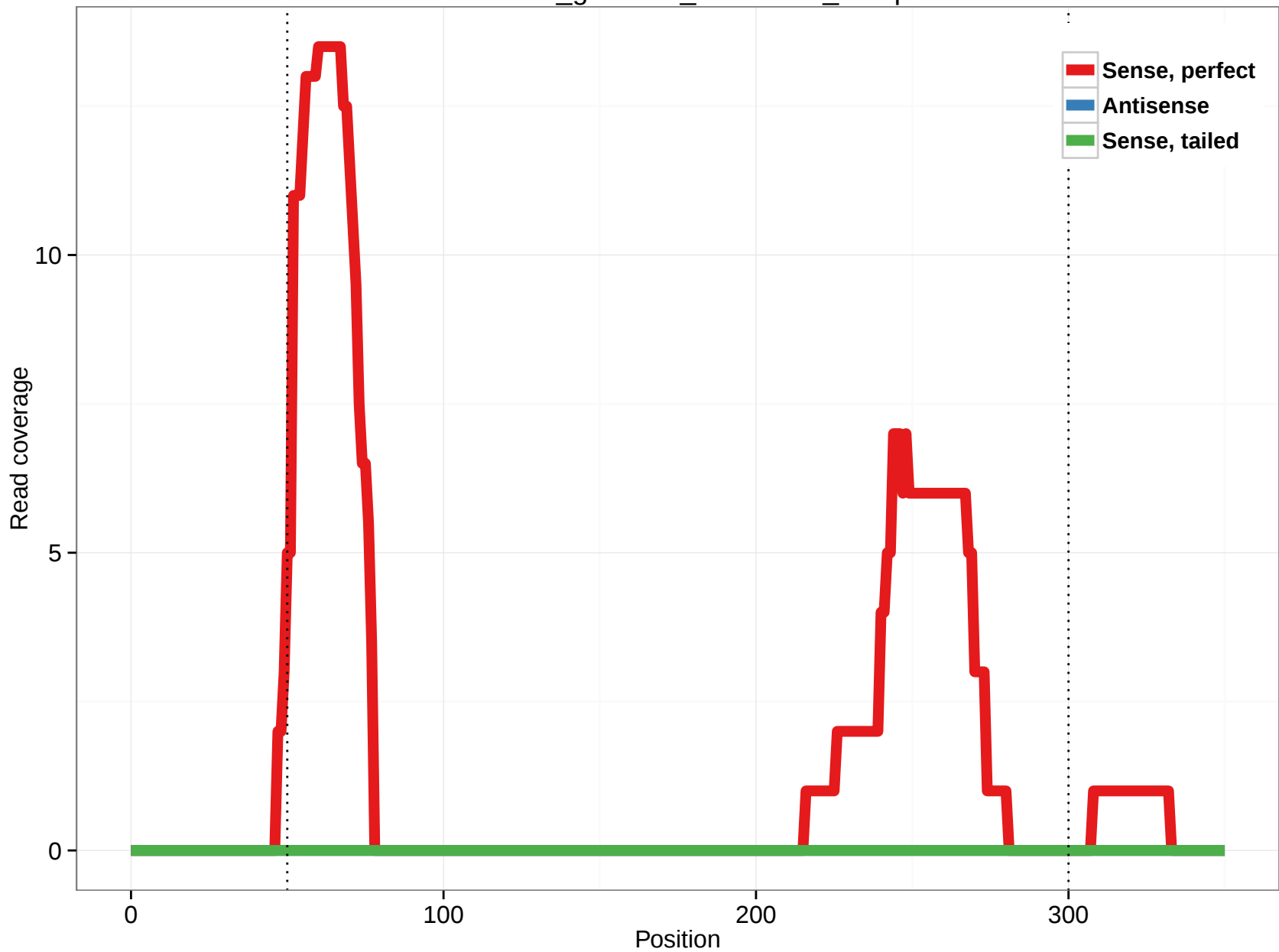
rheMac3_genscan_chr2.3032_41.3p
