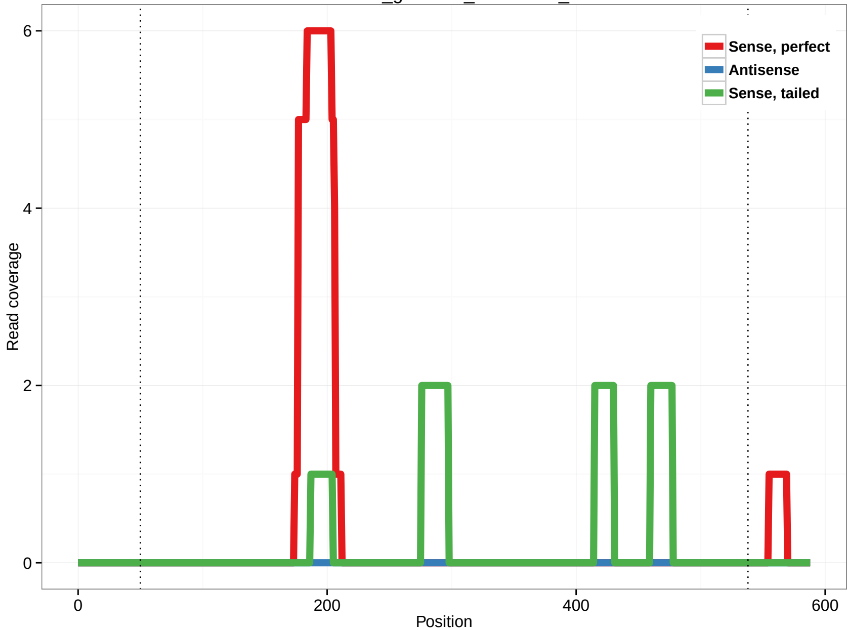
rheMac3_genscan_chr2.3031_5
