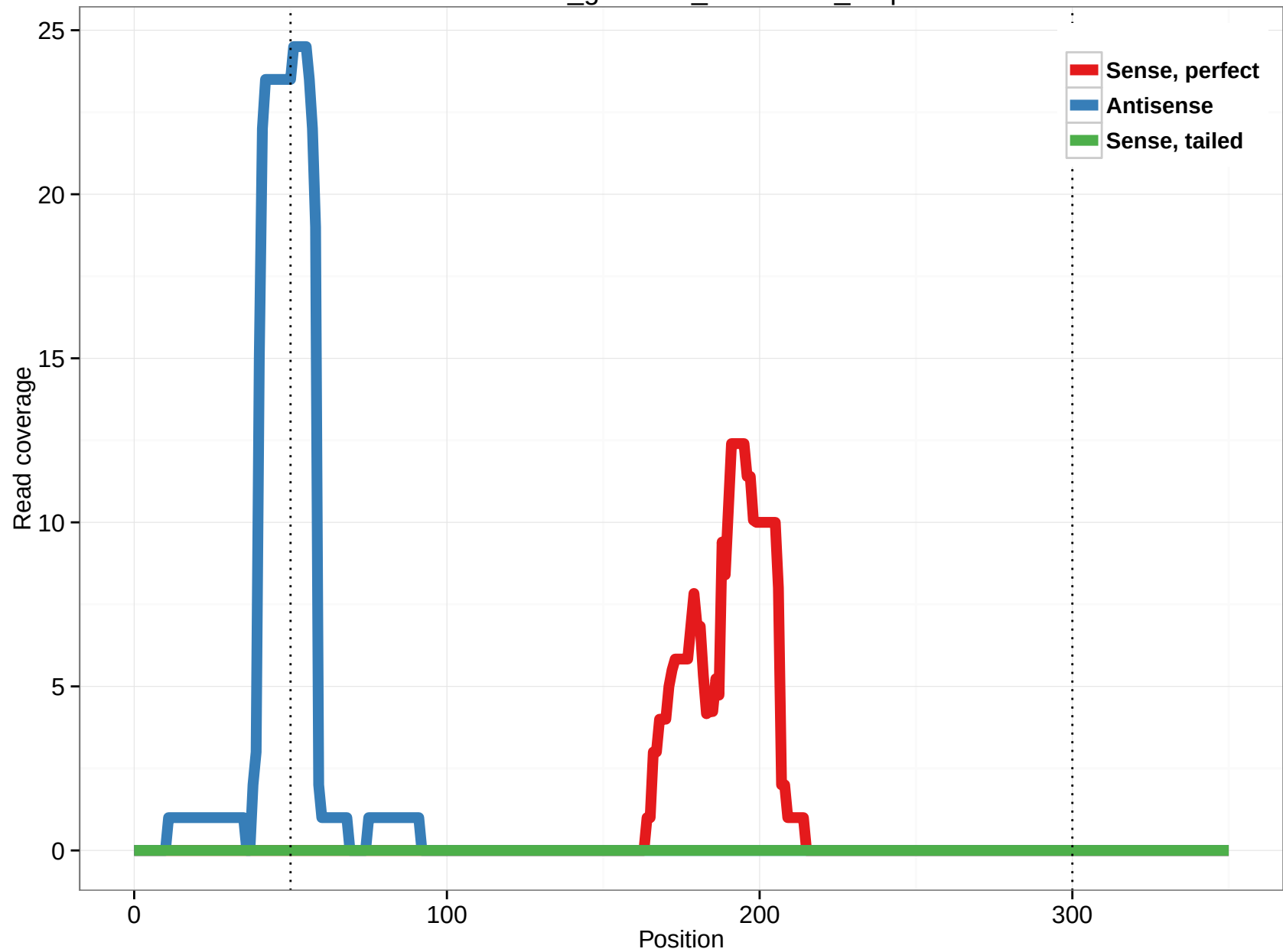
rheMac3_genscan_chr2.2893_1.5p
