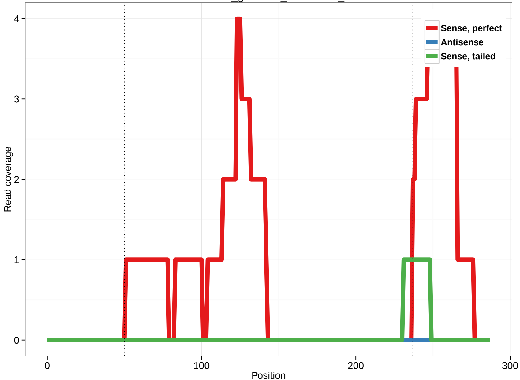
rheMac3_genscan_chr2.2722_0
