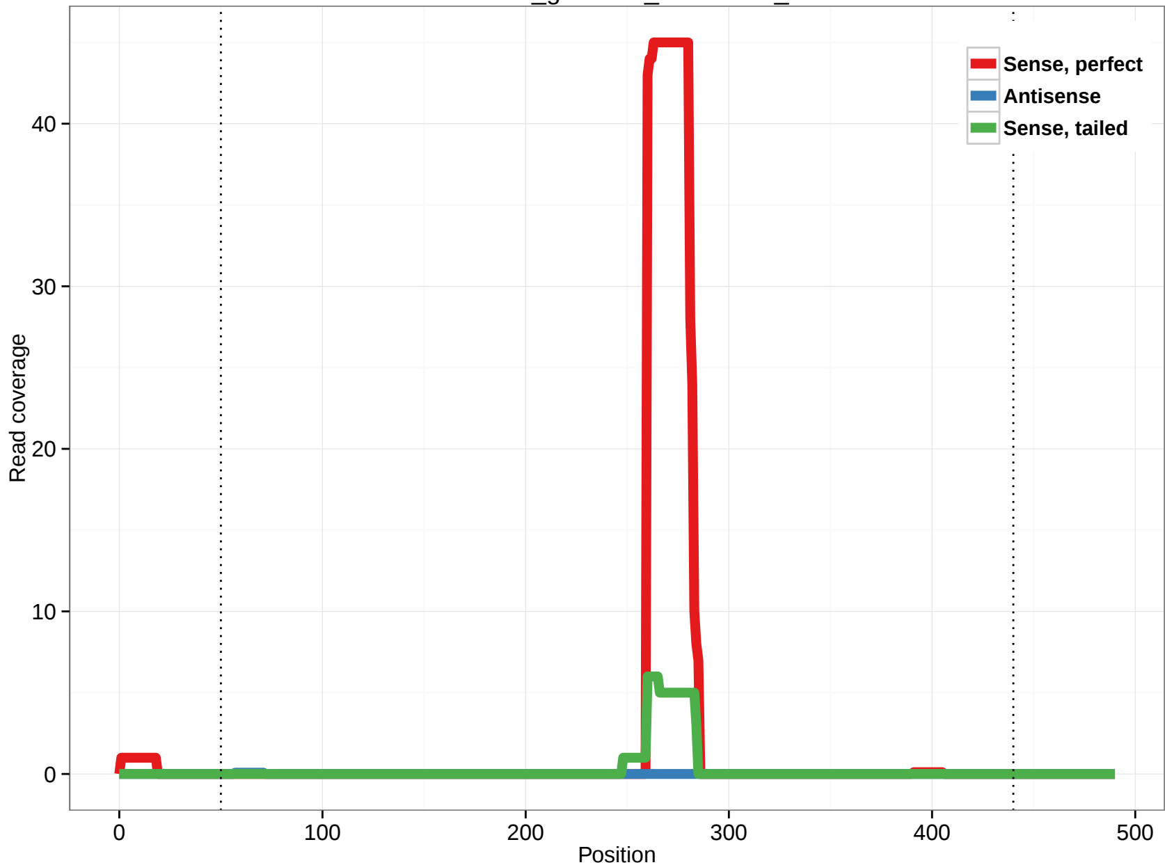
rheMac3_genscan_chr2.2623_2
