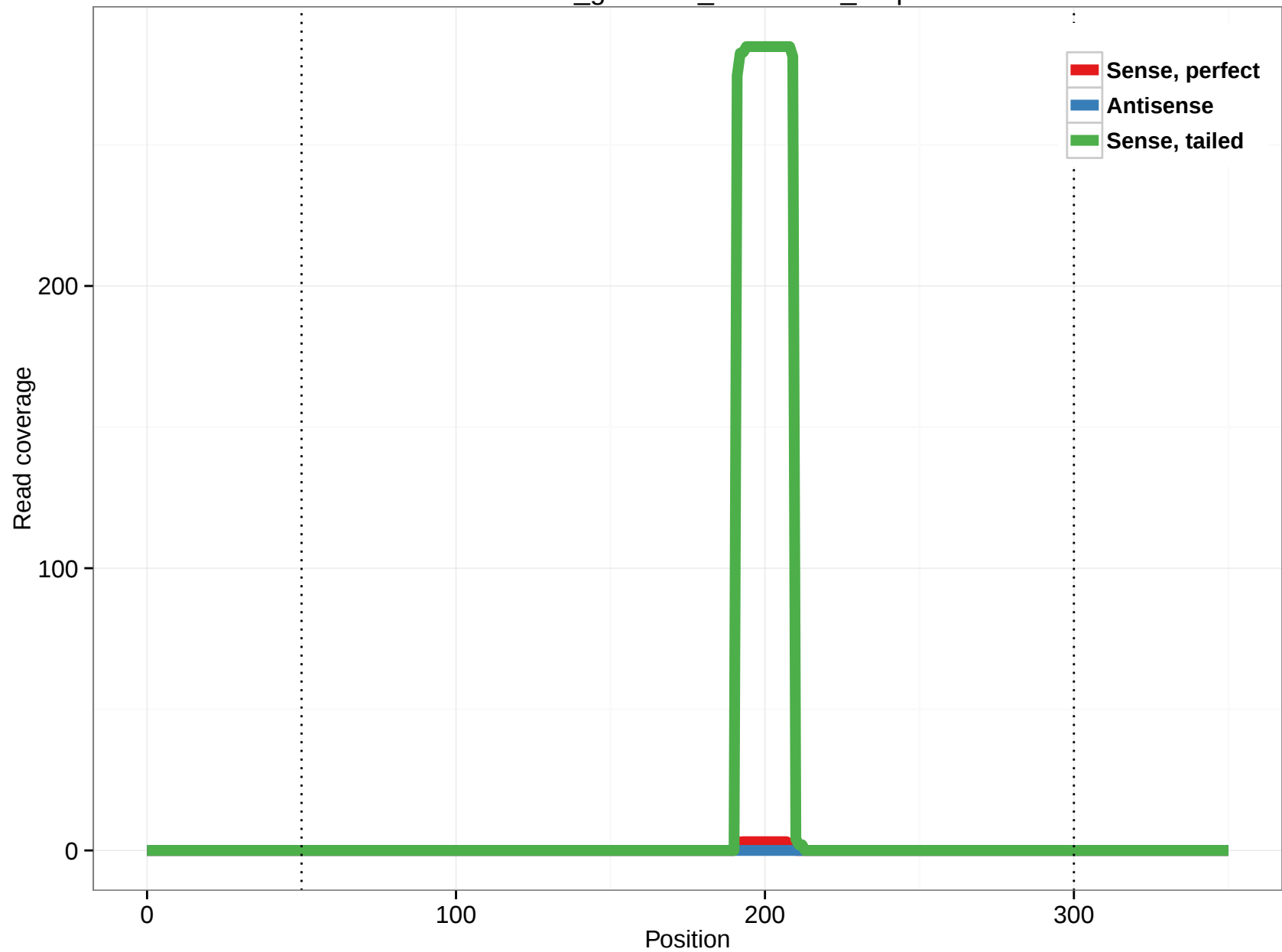
rheMac3_genscan_chr2.2603_1.3p
