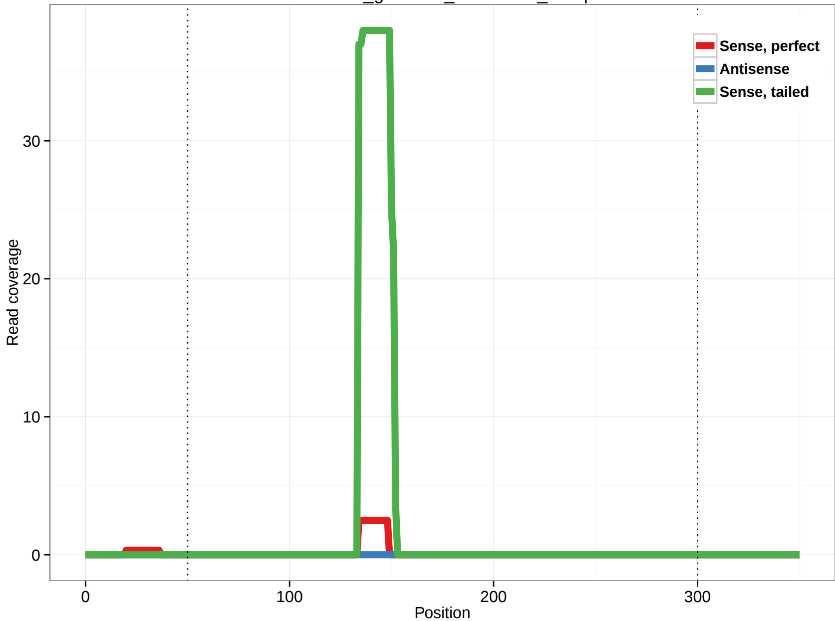
rheMac3_genscan_chr2.2575_15.5p
