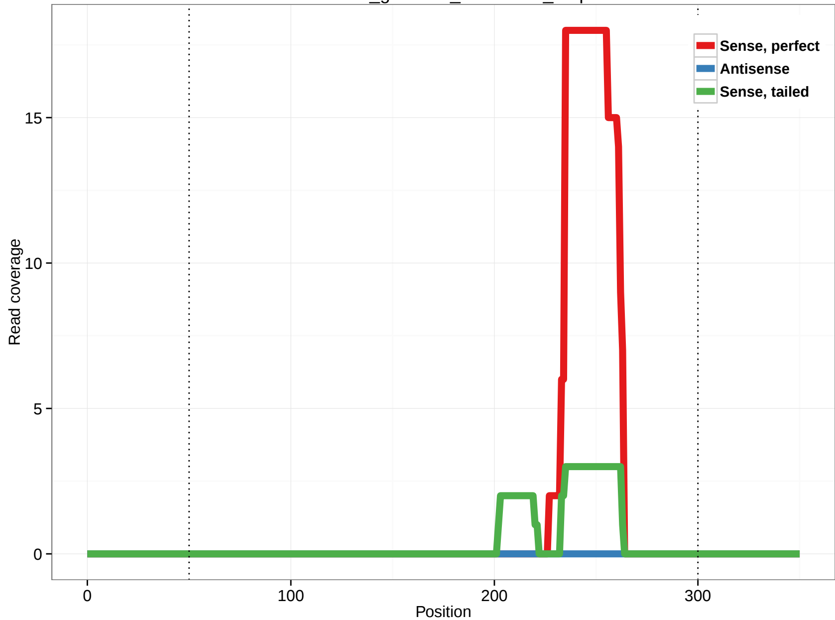
rheMac3_genscan_chr2.2537_8.3p
