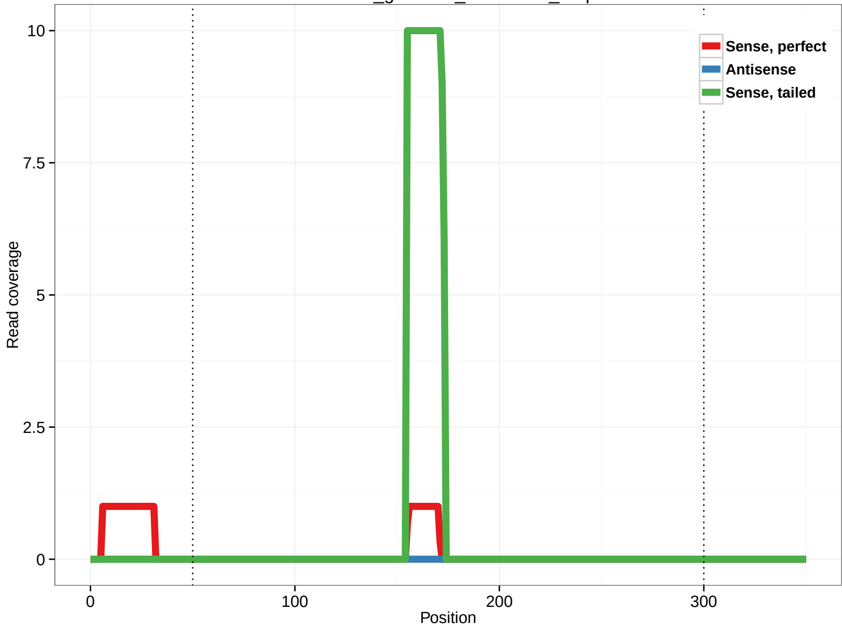
rheMac3_genscan_chr2.2488_7.5p
