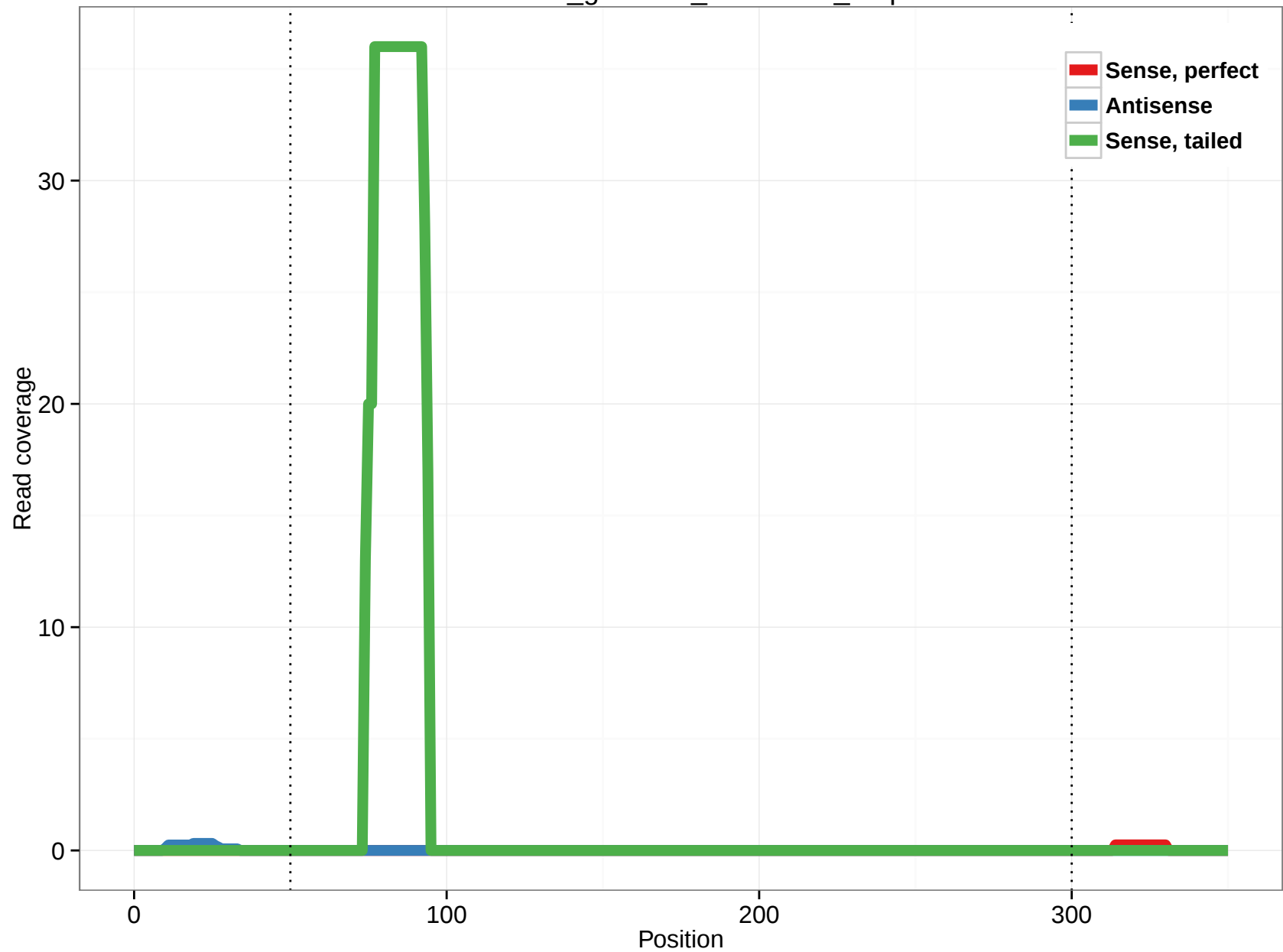
rheMac3_genscan_chr2.2404_7.5p
