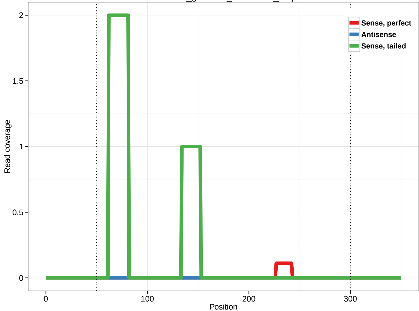
rheMac3_genscan_chr2.2403_7.3p
