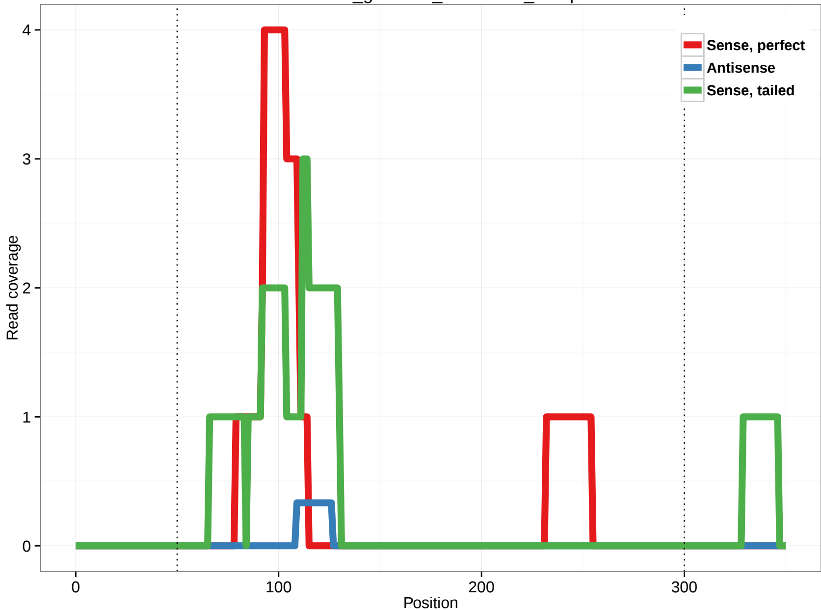
rheMac3_genscan_chr2.2381_10.5p
