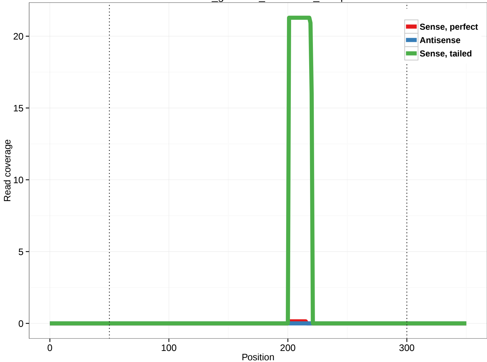
rheMac3_genscan_chr2.2204_16.5p
