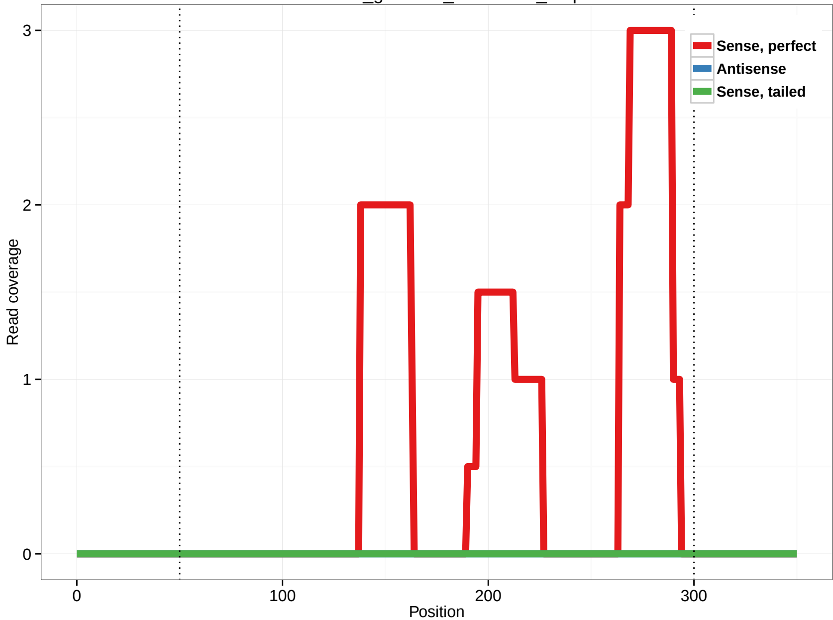
rheMac3_genscan_chr2.2143_0.5p
