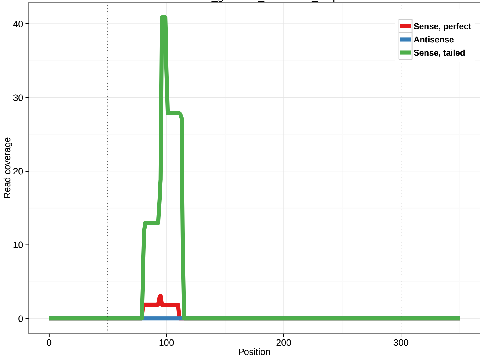
rheMac3_genscan_chr2.2057_1.5p
