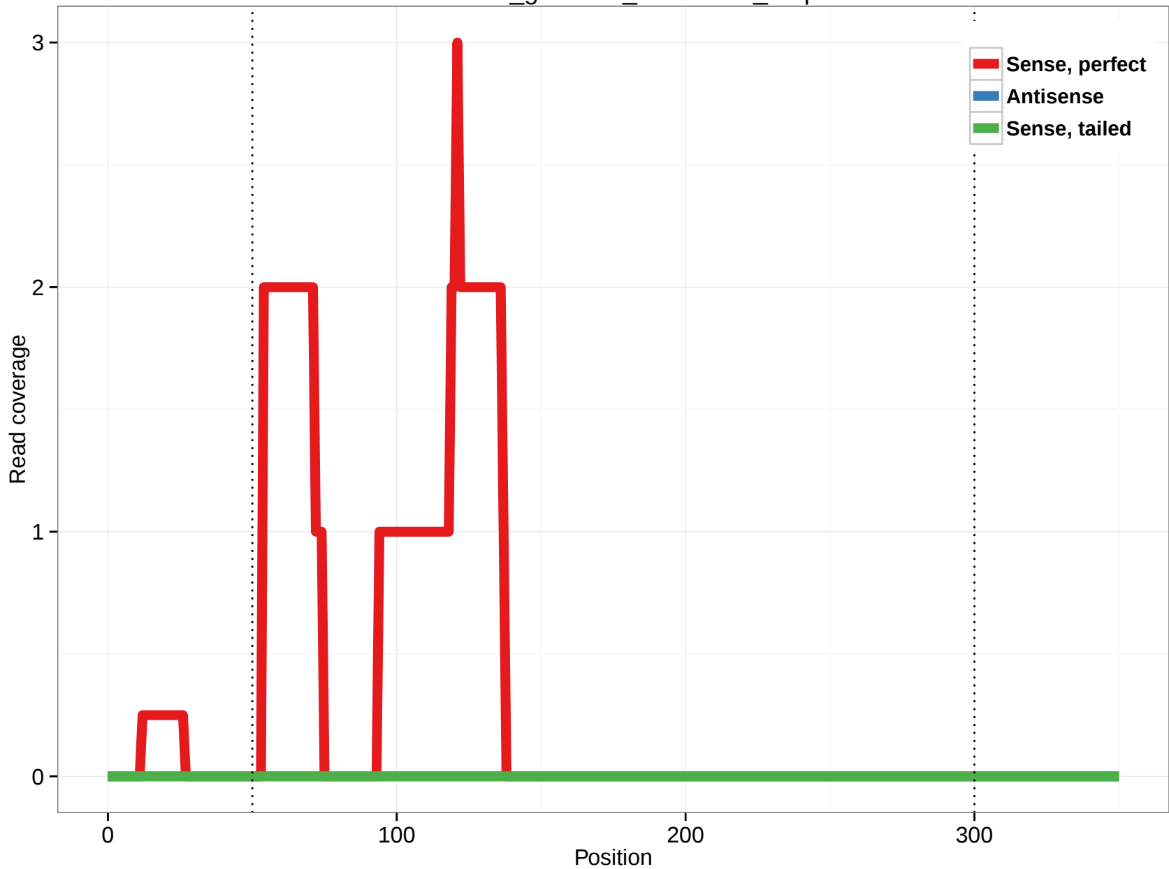
rheMac3_genscan_chr2.2054_0.3p
