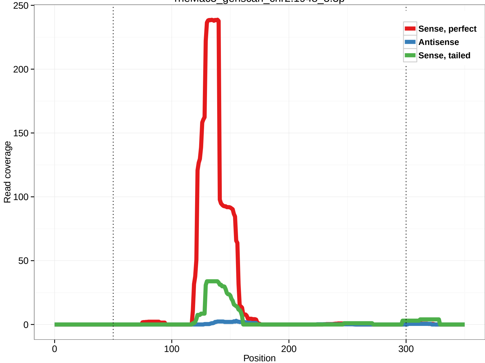
rheMac3_genscan_chr2.1948_3.3p
