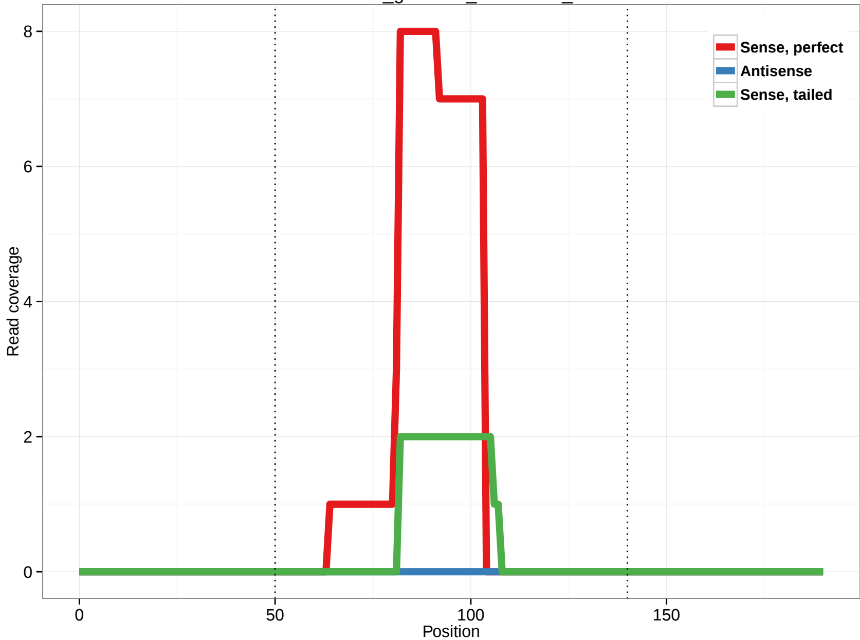
rheMac3_genscan_chr2.1796_20
