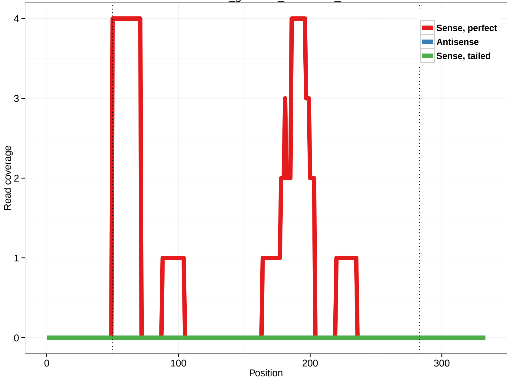
rheMac3_genscan_chr2.1789_3
