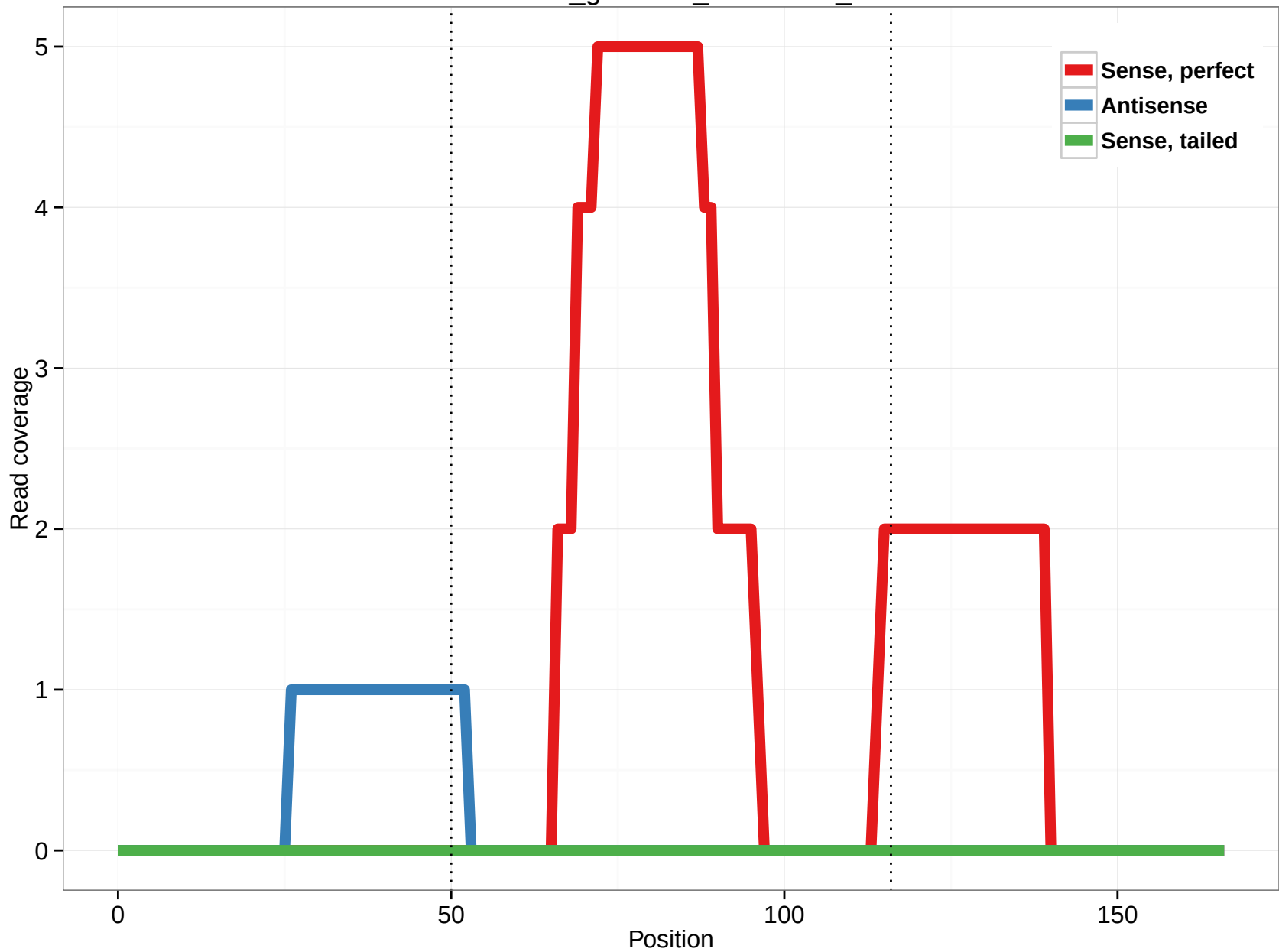
rheMac3_genscan_chr2.1789_15
