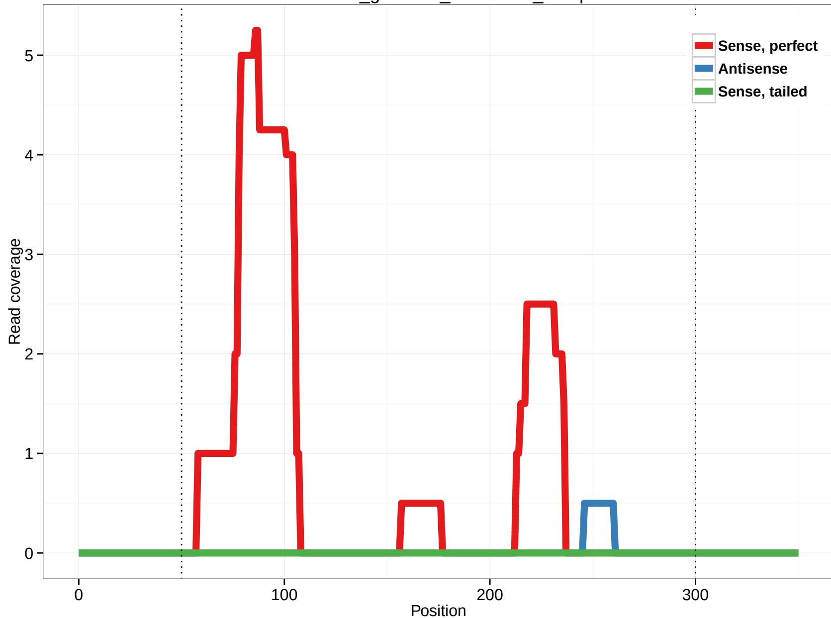
rheMac3_genscan_chr2.1786_37.5p
