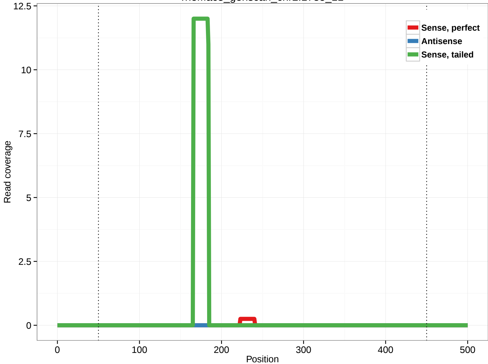
rheMac3_genscan_chr2.1785_11
