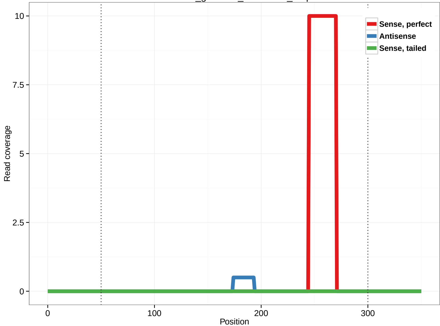
rheMac3_genscan_chr2.1774_0.3p
