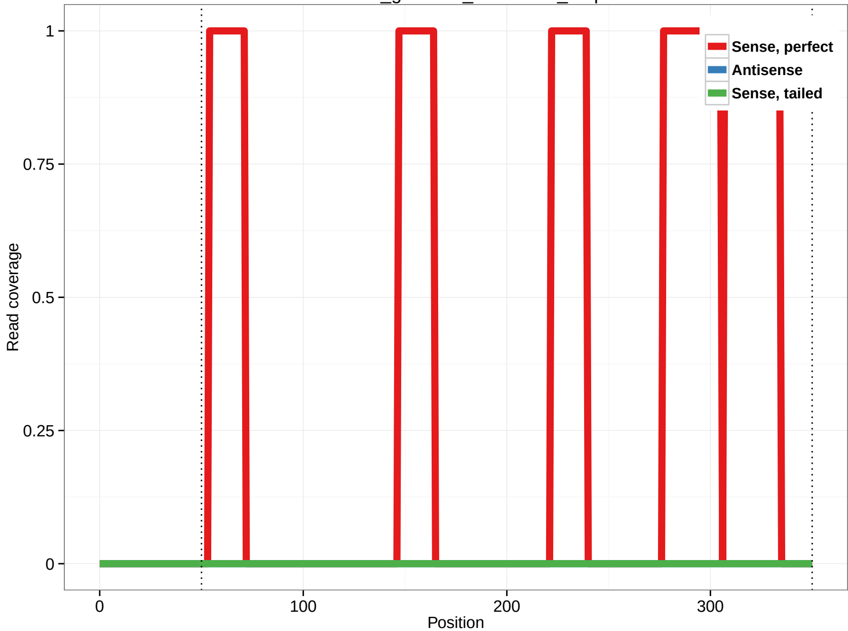
rheMac3_genscan_chr2.1711_4.5p
