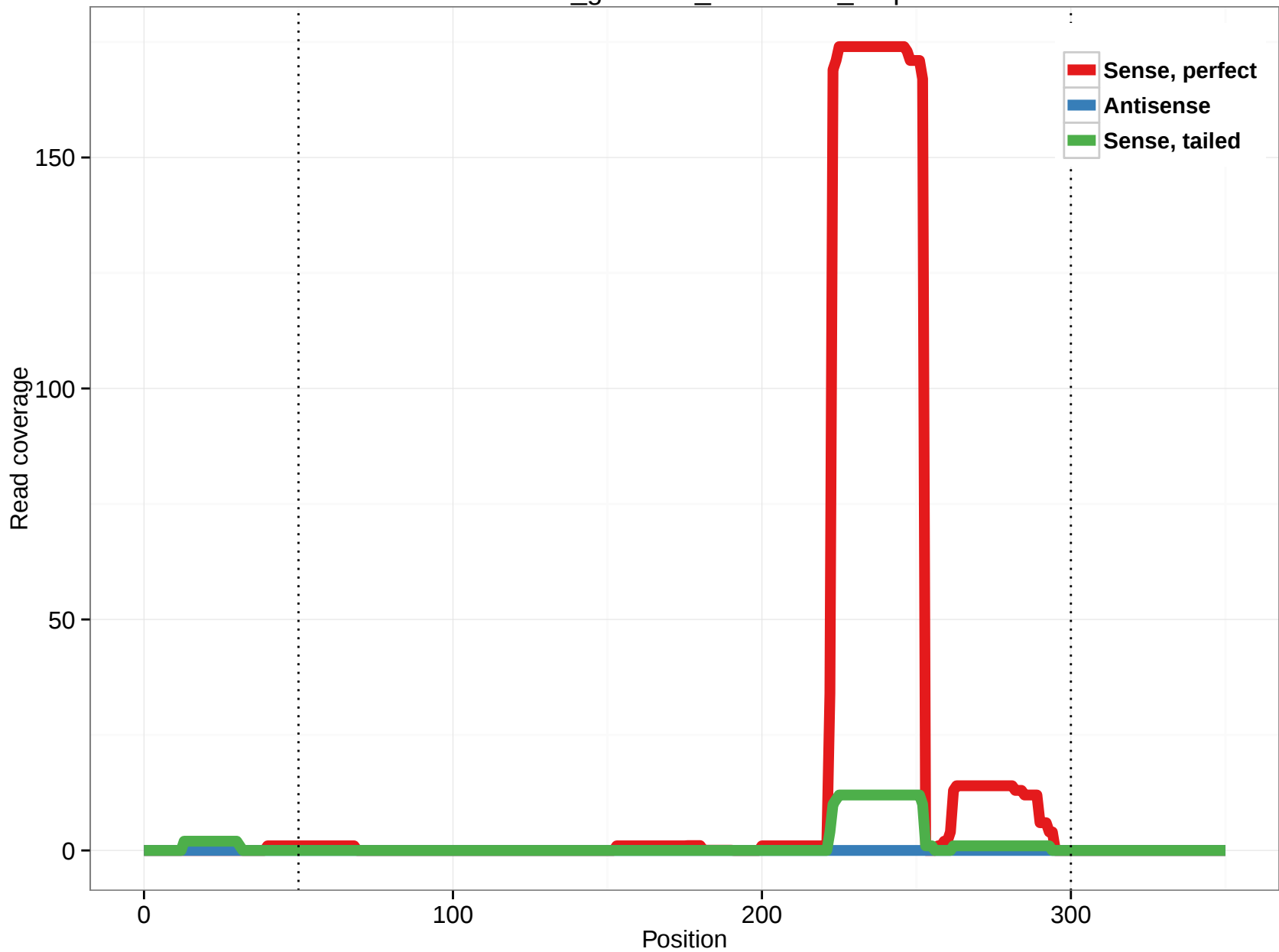
rheMac3_genscan_chr2.1707_2.5p
