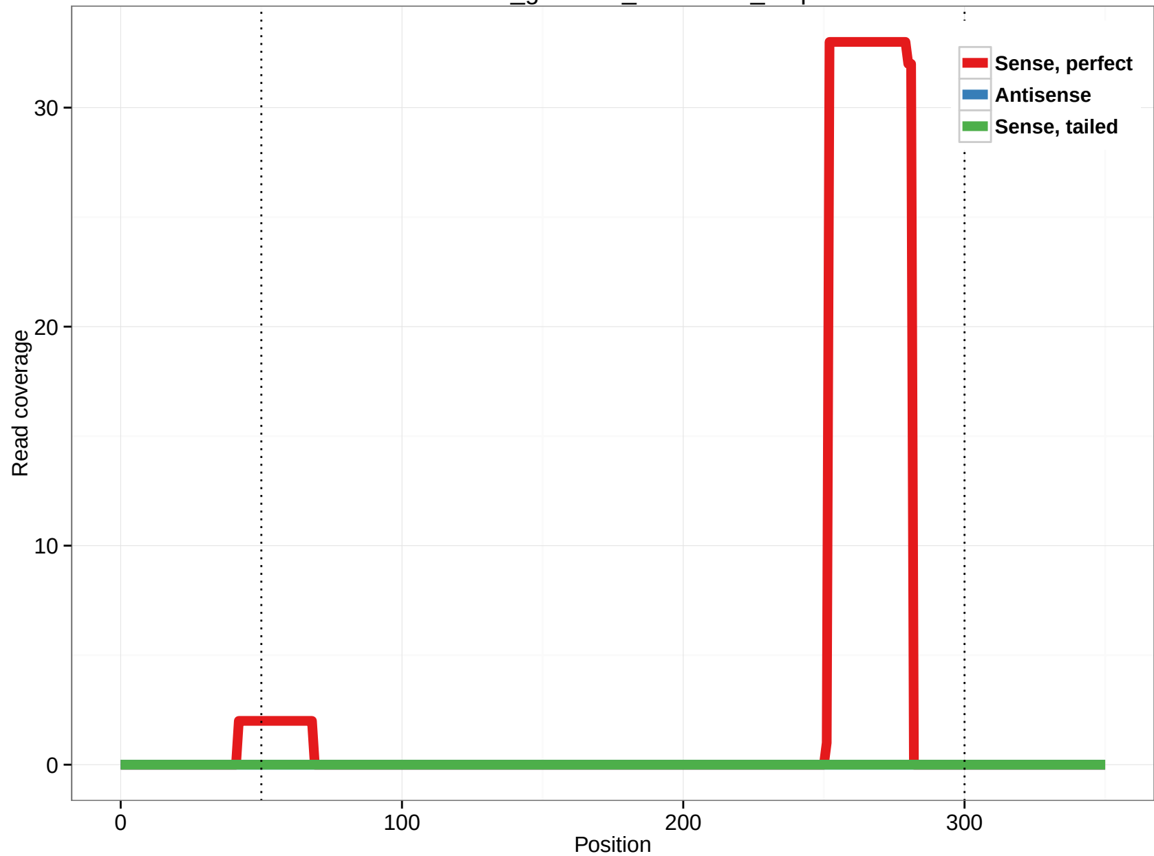
rheMac3_genscan_chr2.1706_9.5p
