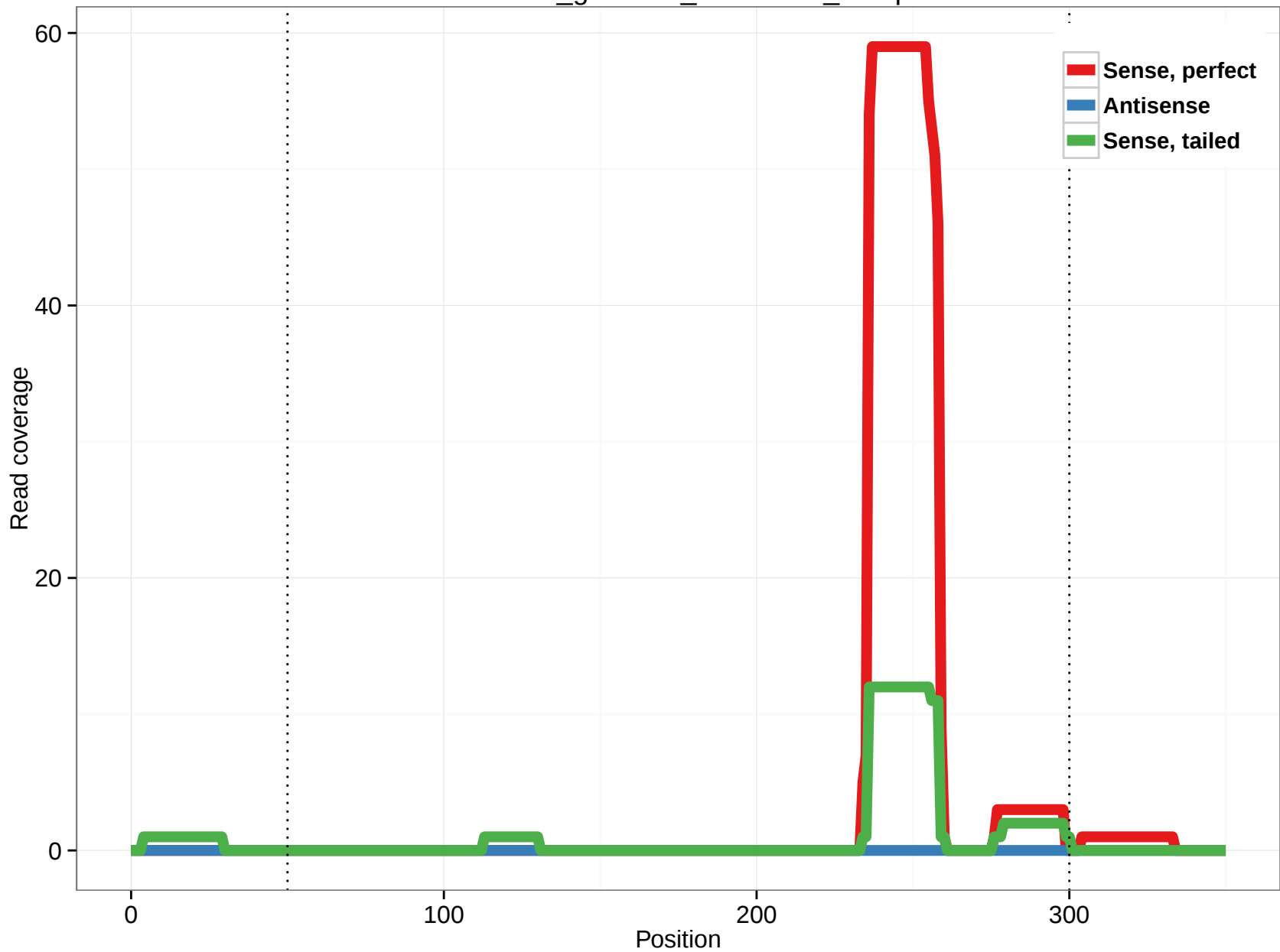
rheMac3_genscan_chr2.1689_38.3p
