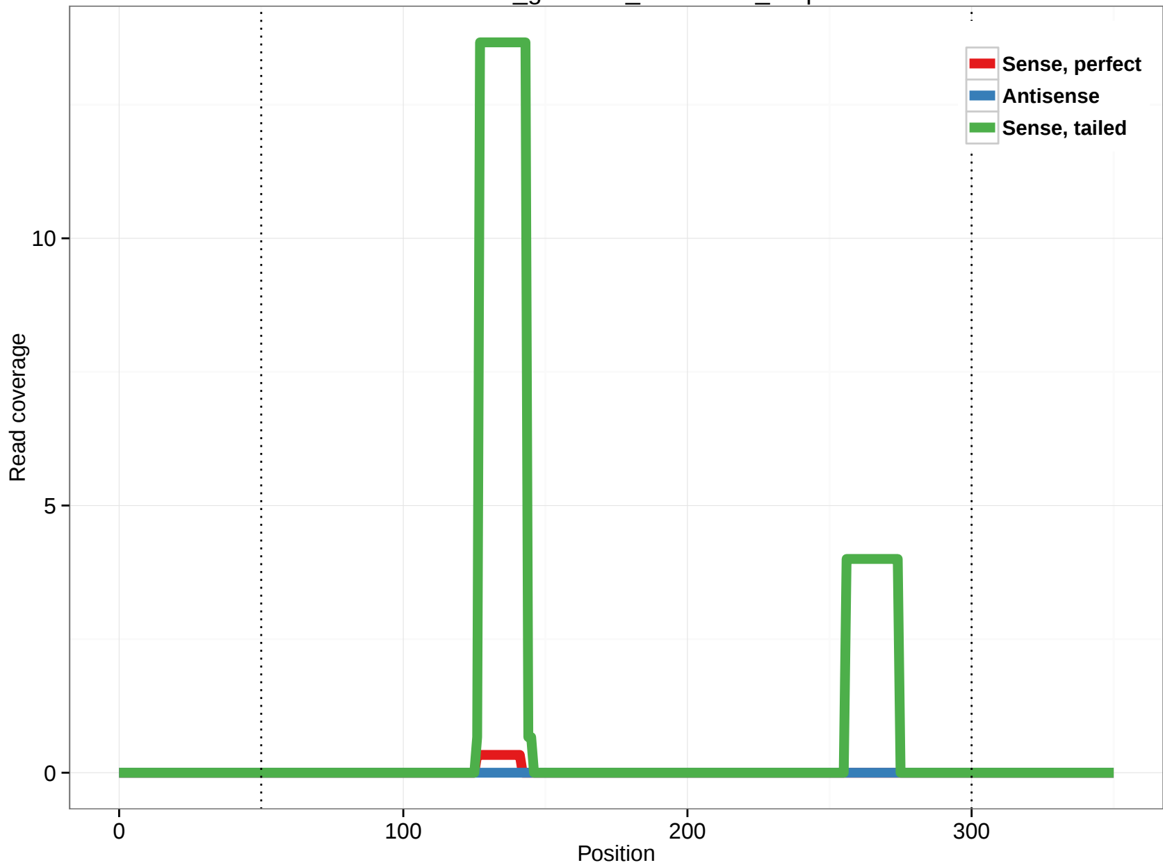
rheMac3_genscan_chr2.1684_9.3p
