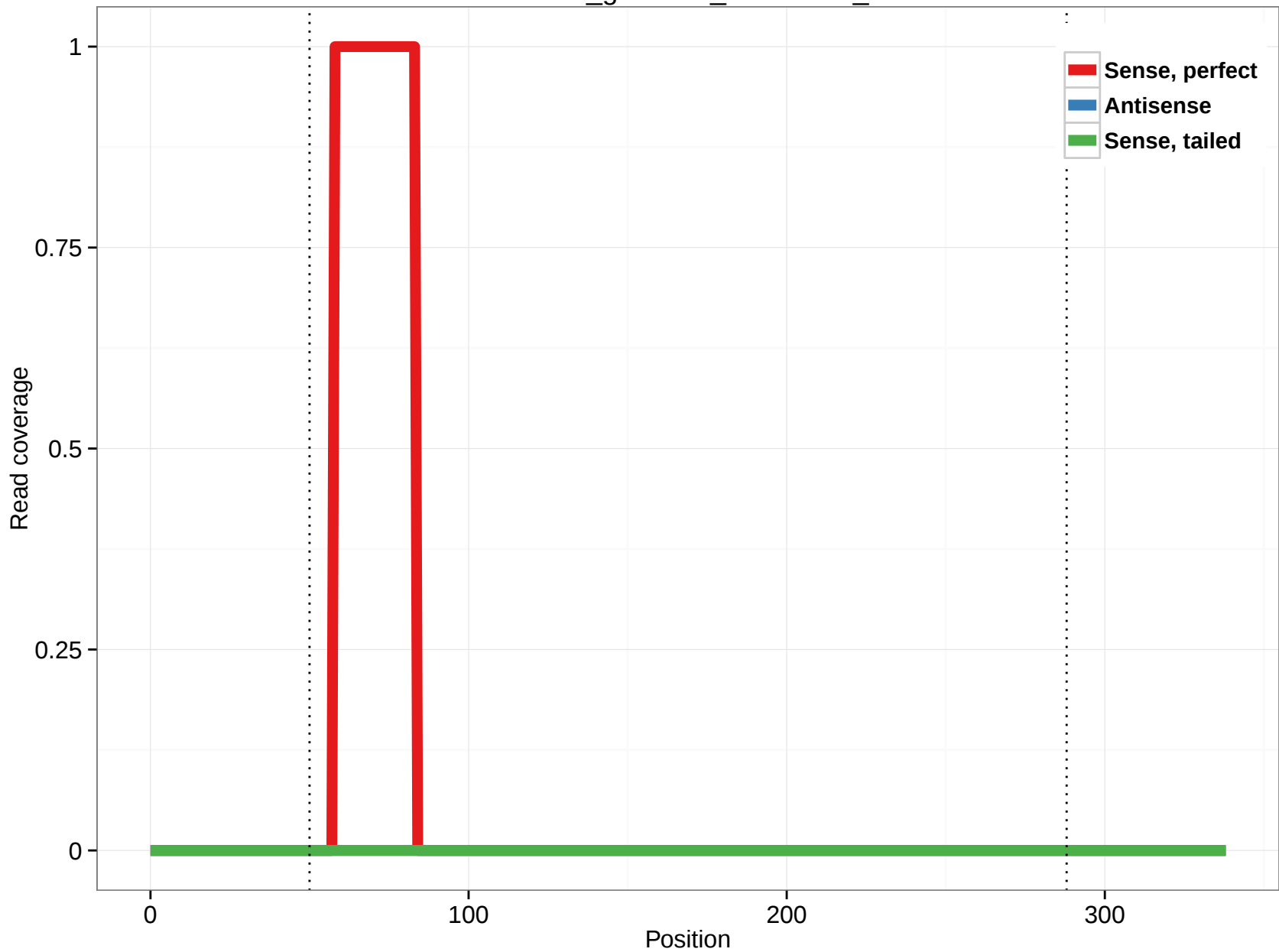
rheMac3_genscan_chr2.1632_18
