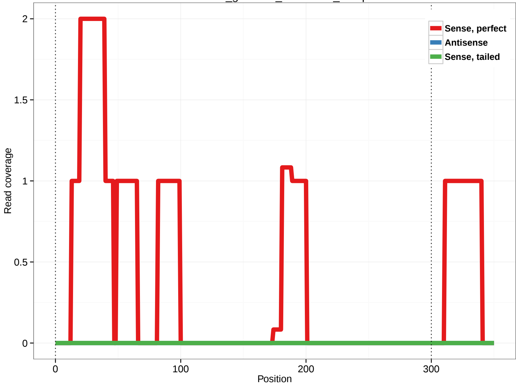
rheMac3_genscan_chr2.1572_23.3p
